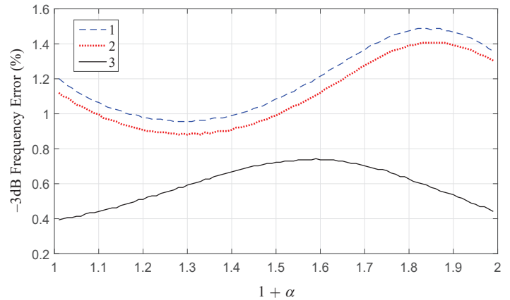
Fig. 5. Percentage error in -3 dB frequency [ k_2 and k_3 varied]: (1) in [10], (2) in [12] and (3) in proposed
