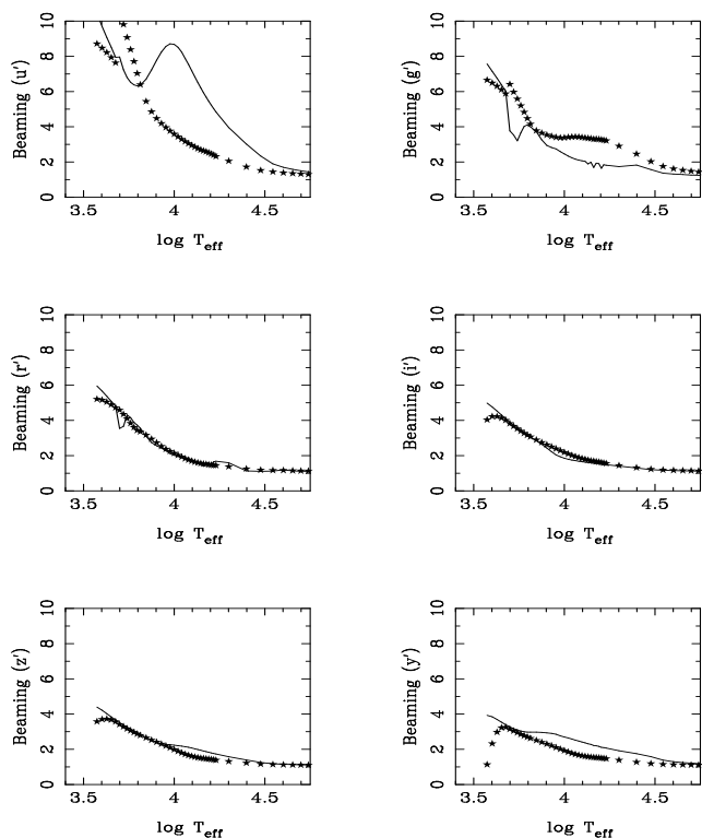
Fig. 2: Comparison between the beaming factors (Sloan passbands, DA white dwarf models) according to Eq. (3). Continuous lines indicate models with \log g = 5.0 while stars denote those with \log g = 9.0 .
