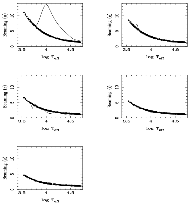
Fig. 1: Comparison between the beaming factors according to Eq. (3) (HiPERCAM passbands). The DA white dwarf models are represented by continuous lines and black body approximation by stars. All models are at \log g = 5.0 .
