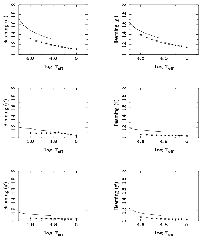
Fig. 4: Beaming factors (Sloan passbands) according to Eq. (3) for \log g=7.0 . Continuous lines indicate LTE DA models and stars indicate NLTE DA models.
