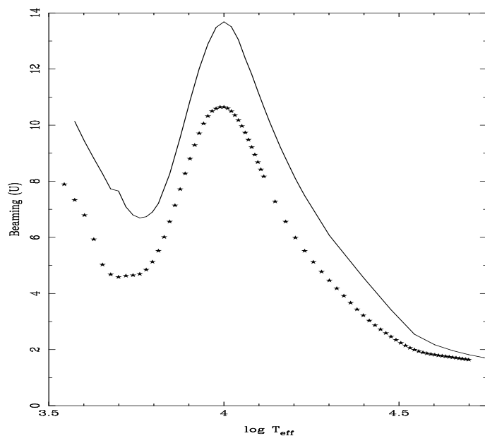
Fig. 6: The same as in Fig. 5 but for the u passband.
