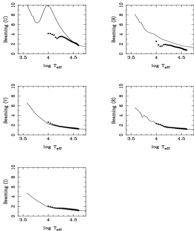
Fig. 3: Beaming factors for the UBVRI passbands according to Eq. (3) for \log g = 5.0 . Continuous lines indicate DA white dwarf models while stars denote DB models.
