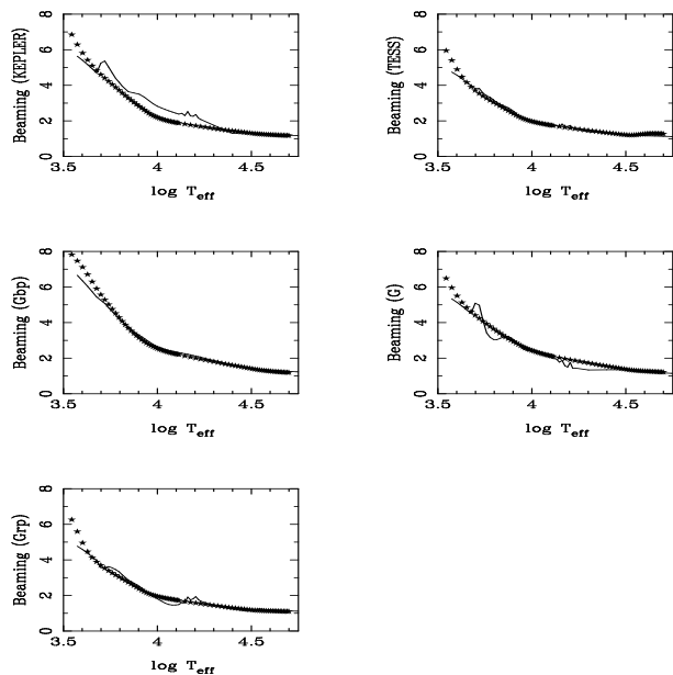
Fig. 5: Beaming factors for main sequence ATLAS9 models (solar metallicity, stars) and DA models (continuous lines) according to Eq. (3). All models are at \log g = 5.0 and shown for the Kepler, TESS and Gaia Gbp, G, and Grp passbands.
