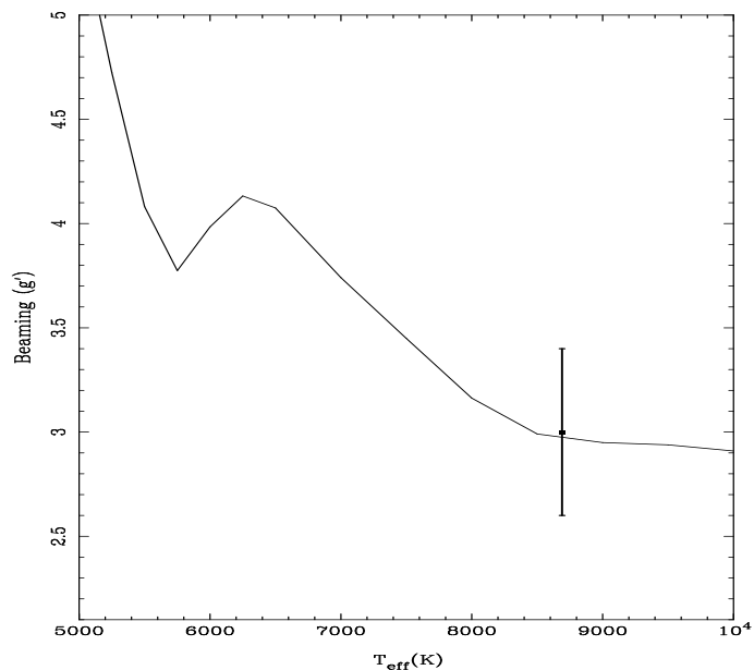
Fig. 7: Comparison between the semi-empirical beaming factor (error bars) for the system NLTT 11748 for the g' passband and theoretical predictions adopting DA models at \log g = 6.5 .
