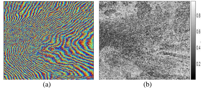
Fig. 13. ERS Interferogram: (a) interferometric phase, (b) coherence coefficient
