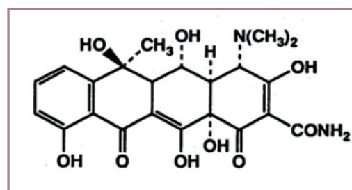
Figure 2.1. Structural formula of oxytetracycline
