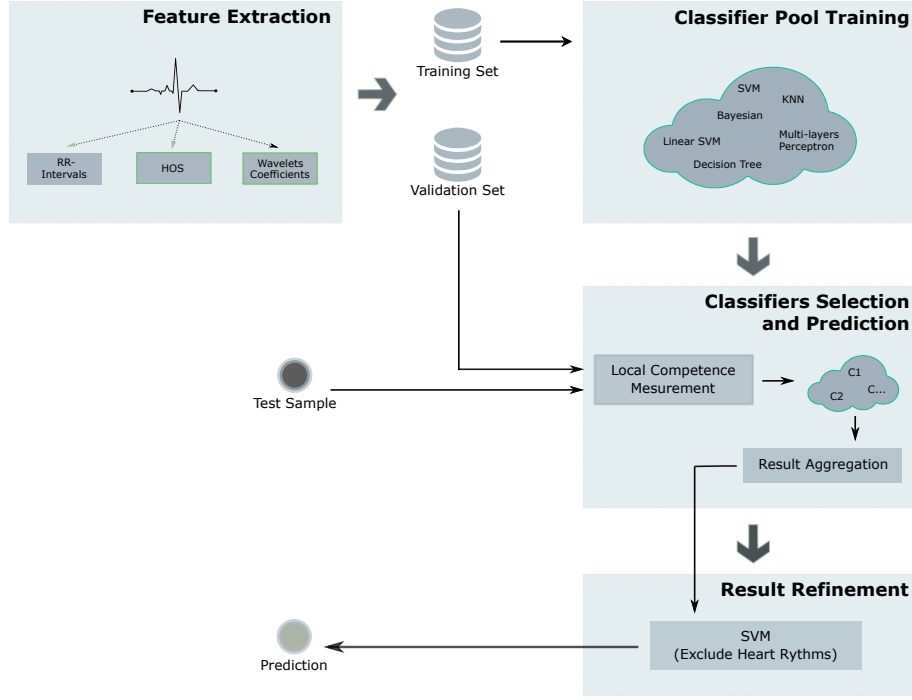
Fig. 3. Architecture of the proposed DHCAF.
