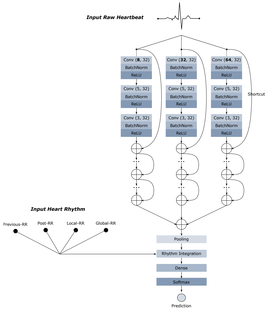
Fig. 4. Architecture of the proposed Multi-channels Heartbeat Convolution Neural Network (MCHCNN).
