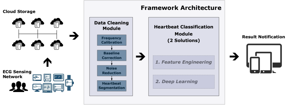
Fig. 2. Architecture of the proposed framework. The whole life-cycle of arrhythmia detection from IoT-based ECGs includes 4 phases: data collection, storage, analysis and results notification. Specifically, ECG sensing network generates ECG recordings for patients and transmits the produced data to the IoT cloud, where fast access storage are conducted. The proposed framework is deployed in the IoT cloud to provide data analysis. Results from the framework will be pushed to patients' ends via Internet.
