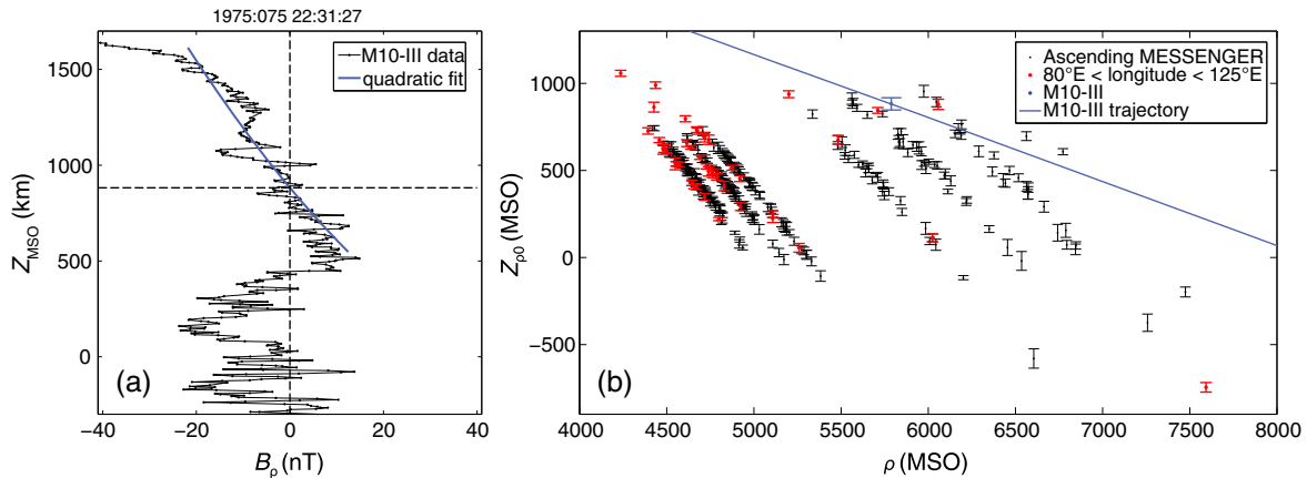
Figure 2. (a) Z_{MSO} versus B_\rho for M10-III near the magnetic equator crossing along with the quadratic function fit to the near-crossing data (solid blue line). The instantaneous equator crossing obtained from the fit is indicated by the dashed lines. The data shown here span the time interval 22:26–22:35 UTC on 16 March 1975. (b) Magnetic equator crossing Z_{\rho 0} versus \rho = (X_{MSO}^2 + Y_{MSO}^2)^{1/2} for M10-III (blue symbol and trajectory) and for the ascending legs of MESSENGER orbits (black symbols) between 24 March 2011 and 15 December 2012. MESSENGER magnetic equator crossings with MSO longitudes similar to that of the M10-III crossing (in the range 80°E to 125°E) are shown in red. Error bars indicate three standard errors.
