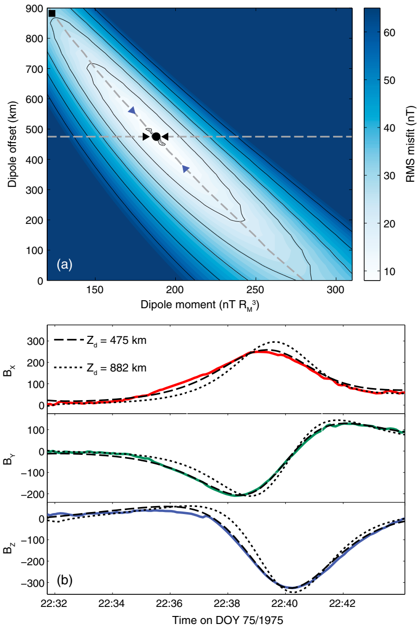
Figure 3. (a) RMS misfit between model and M10-III data obtained from a grid search over dipole moment and offset of the dipole from the geographic equator. Contours indicate misfits from 10 nT to 60 nT in 10 nT steps. The parameter pairs for the best fit offset of Z_d = 475 km and the M10-III magnetic equator offset of 882 km are marked by the filled black circle and filled square, respectively. The diagonal dashed line shows the trade-off between best fit dipole offset and dipole moment; blue triangles correspond to parameter pairs that yield an RMS misfit 25% above the minimum value. The horizontal dashed line shows the location of an RMS misfit profile corresponding to the best fit dipole offset; a 25% increase above the minimum misfit would yield dipole moments shown by the black triangles. (b) Magnetic field observations from M10-III inside the magnetopause (solid lines) and best fit models to the data for dipole offsets of 475 km (dashed line) and 882 km (dotted line).
