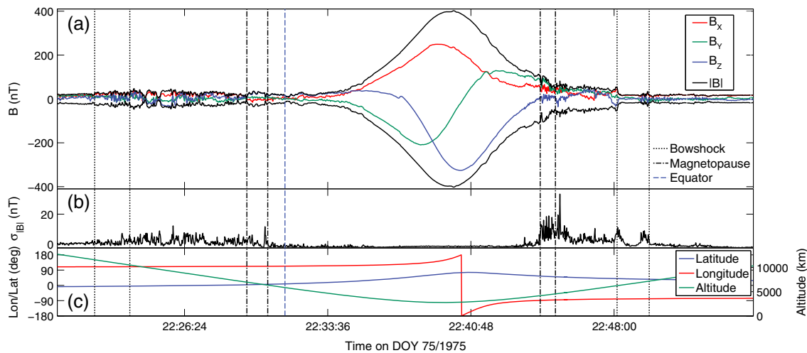
Figure 1. M10-III data in MSO coordinates. (a) Magnetic field components and magnitude averaged over 1.2 s intervals; crossing times for the magnetopause, bow shock, and magnetic equator are indicated by vertical lines. (b) Standard deviation in total magnetic field, \sigma_{|B|} , over the averaging interval and spacecraft position in MSO coordinates and altitude. The magnetopause and inner and outer bow shock crossings for each boundary were identified by the methodology of Winslow et al. [2013], using the vector field, \mathbf{B} , and \sigma_{|B|} . DOY is day of the year.
