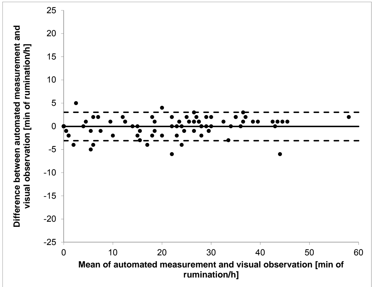
Figure 1: Agreement of automated RumiWatch noseband sensor measurements and visual observations of feeding behaviour (a) grazing and (b) rumination time in 1-hour periods, displayed in Bland-Altman-plots ( solid line indicates the mean difference; dashed lines indicate upper and lower 95% limits of agreement ).
