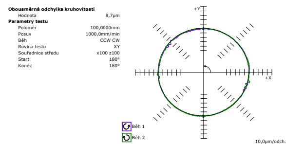
Figure 3. Roundness deviation in XY plane - first measurement
