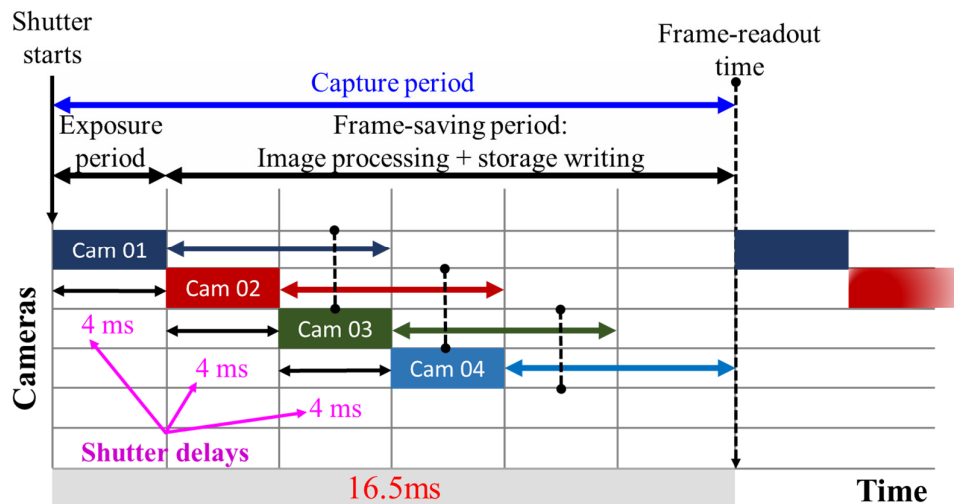
Figure 34. Timed shutter for multiple-camera frame rates.
