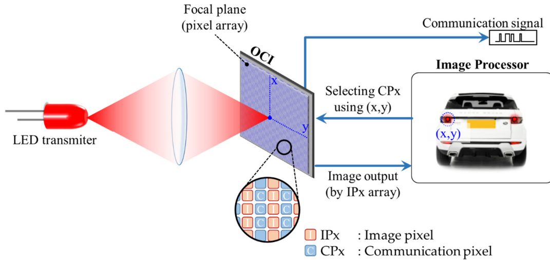
Figure 19. Basic operation of IS-OWC system.
