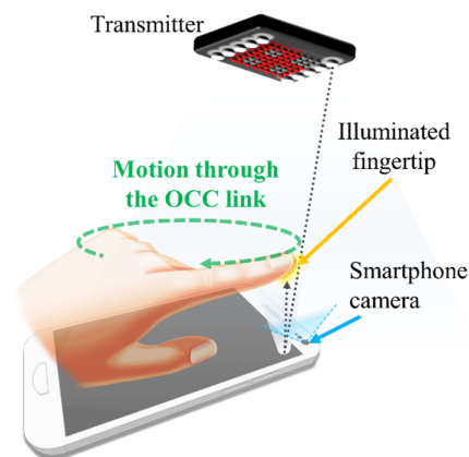
Figure 29. A motion over camera scheme.
