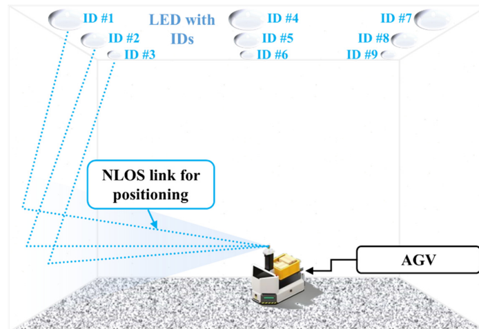
Figure 36. AGV potential indoor positioning scheme.
