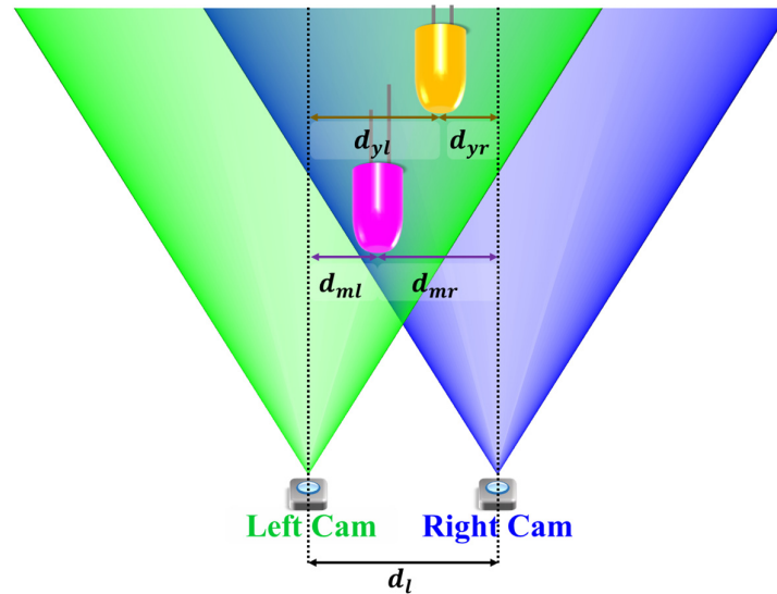
Figure 35. Stereoscopic vision for distance measurement.
