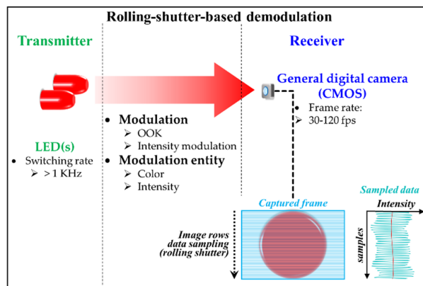
Figure 20. RS-based demodulation process.
