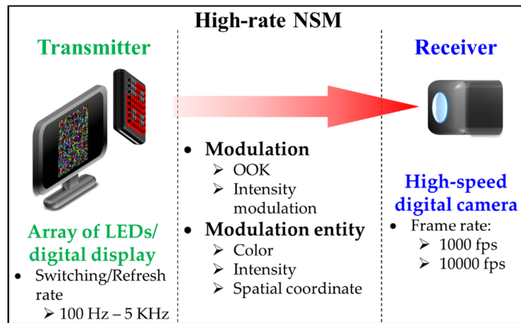
Figure 16. High-rate Nyquist sampling modulation (NSM).
