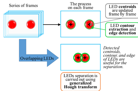
Figure 28. Detection algorithm for overlapping LEDs [92].
