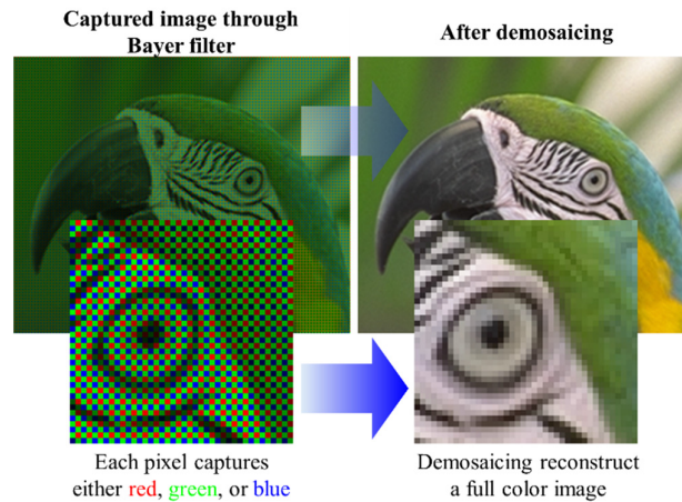
Figure 7. An example of the demosaicing process.
