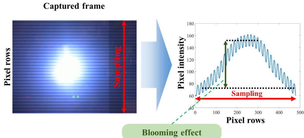
Figure 22. Blooming effect on RS-OCC.
