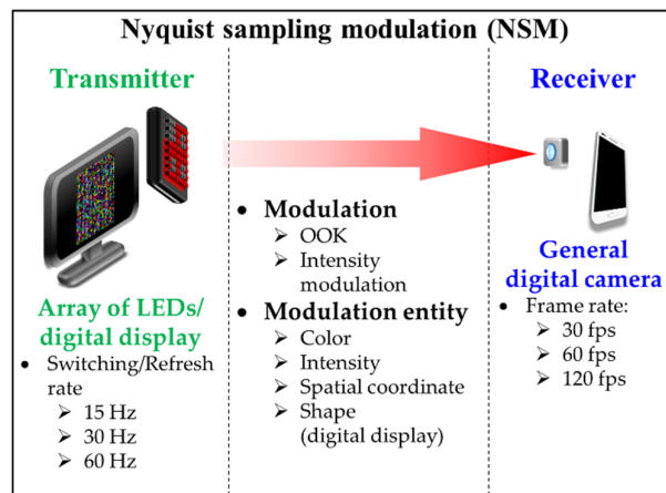
Figure 13. Nyquist sampling modulation.
