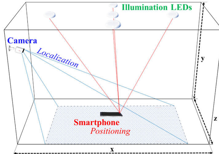
Figure 31. Indoor positioning schemes for OCC.
