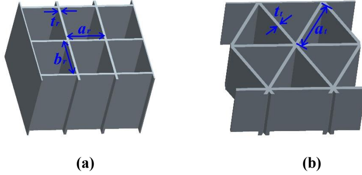
Fig. 2 Top view of sandwich panel with (a) rectangular core and (b) triangular core
