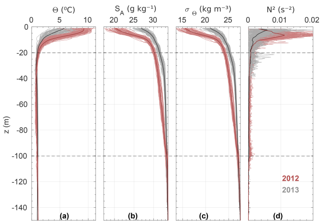
Figure 5. (a) Conservative temperature, (b) absolute salinity, (c) sigma-theta (potential density - 1000 \text{ kg m}^{-3} ) and (d) squared Brunt–Väisälä frequency profiles (Eq. 1) derived from CTD casts in Saqqarleq fjord during field surveys in July 2012 (red) and 2013 (grey). Averaged profiles are shown as darker lines and are used as ambient boundary conditions for the line plume model. Casts from inside the plume are not included here. Note that the water column is characterized in three layers separated by dashed horizontal lines.
