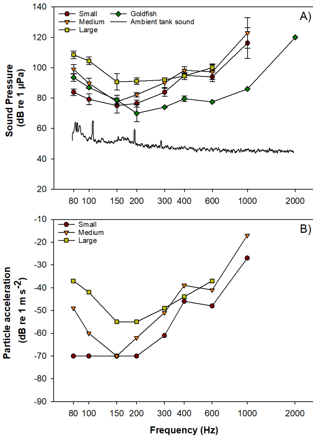
Figure 2. Sound pressure levels and measured particle acceleration at auditory thresholds of Centropomus striata (n=20) and Carassius auratus (n=4). A) Mean ( \pm SE) sound pressure levels at auditory thresholds for three size classes of C. striata and C. auratus , and ambient sound pressure levels of AEP tank, B) Particle acceleration levels measured at identified auditory thresholds. Flat response for the Small size class at frequencies 80 – 200 Hz due to noise floor of accelerometer. The ambient tank sound was also below the noise floor of the accelerometer.
