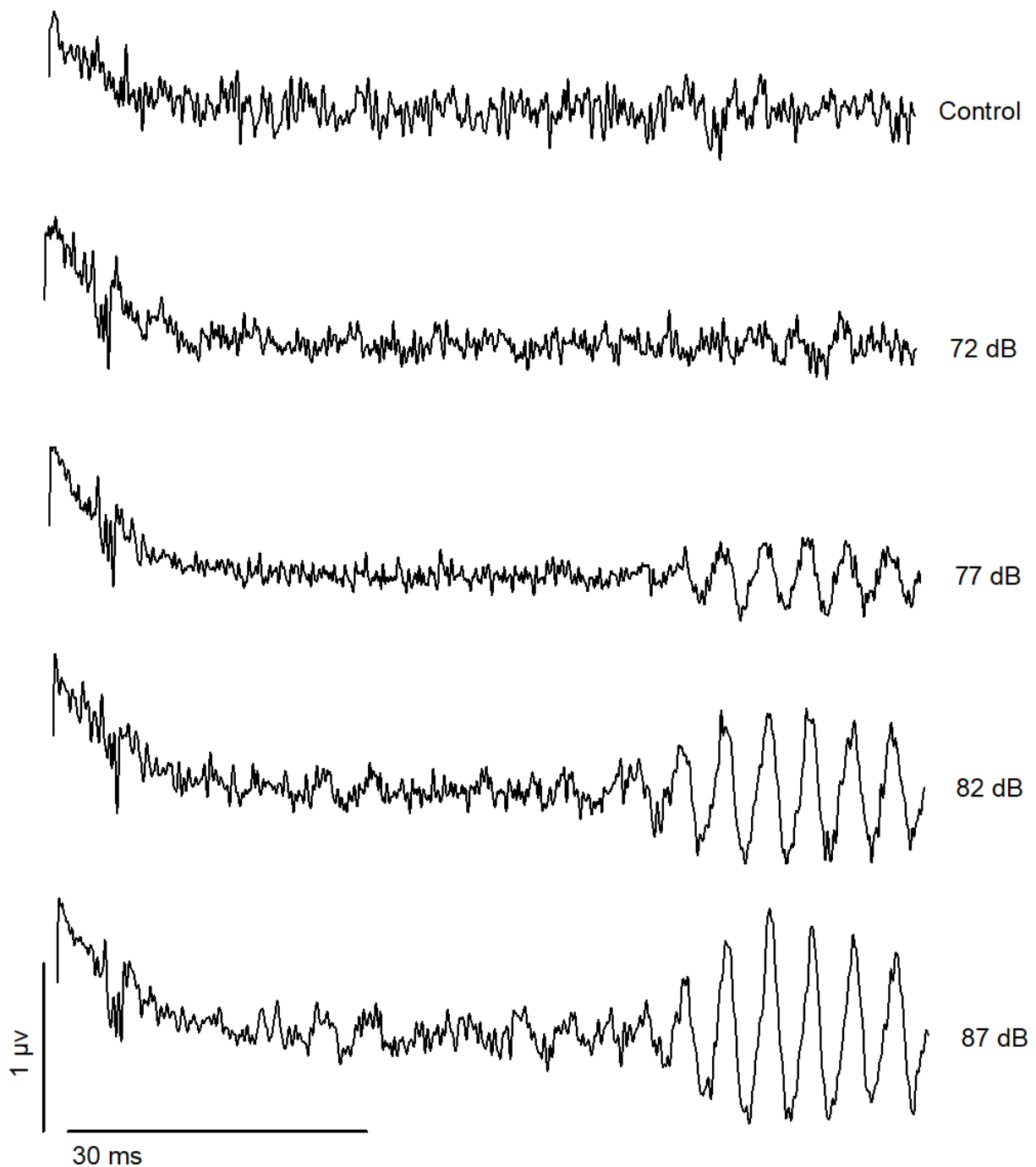
Figure 1. Example of auditory evoked potential waveforms from an individual Centropristis striata (93 mm TL) from the Small size class, in response to sound stimulus of 100 Hz pure tone bursts. The lowest sound pressure level to show a definitive response occurred at 77 dB in this example. Stimulus duration in this example was 30 ms, as indicated by the black bar in the lower left. Control AEPs (as shown here) were performed with a euthanized fish.
