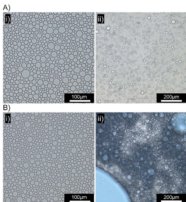
Fig. 6 Optical microscopy images of squalene-in-water emulsions containing Oil Blue A (0.1 wt%). (A) [Dod 1.00 ]- p (OEGMA 50-co -EGDMA 0.80 )- and (B) [SH 0.75 /Dod 0.25 ]- p (OEGMA 50-co -EGDMA 0.80 )-stabilised emulsions both (i) before and (ii) 10 minutes after addition to a biosimilar mucosal surface.
