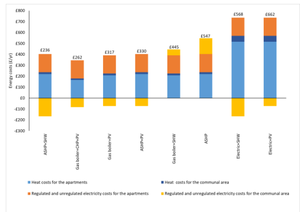
Figure 3: Apartment energy cost including heat, regulated and unregulated electricity
