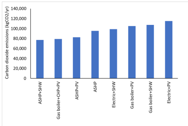
Figure 4: Annual CO 2 emissions based on regulated energy for the entire development (residential and communal areas).
