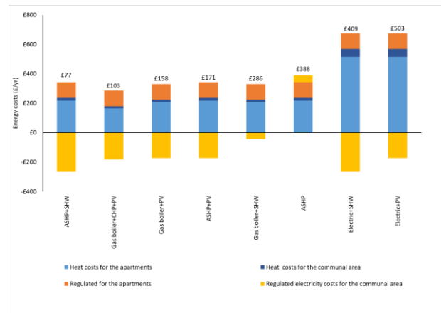
Figure 2: Apartment energy costs including heat and regulated electricity only
