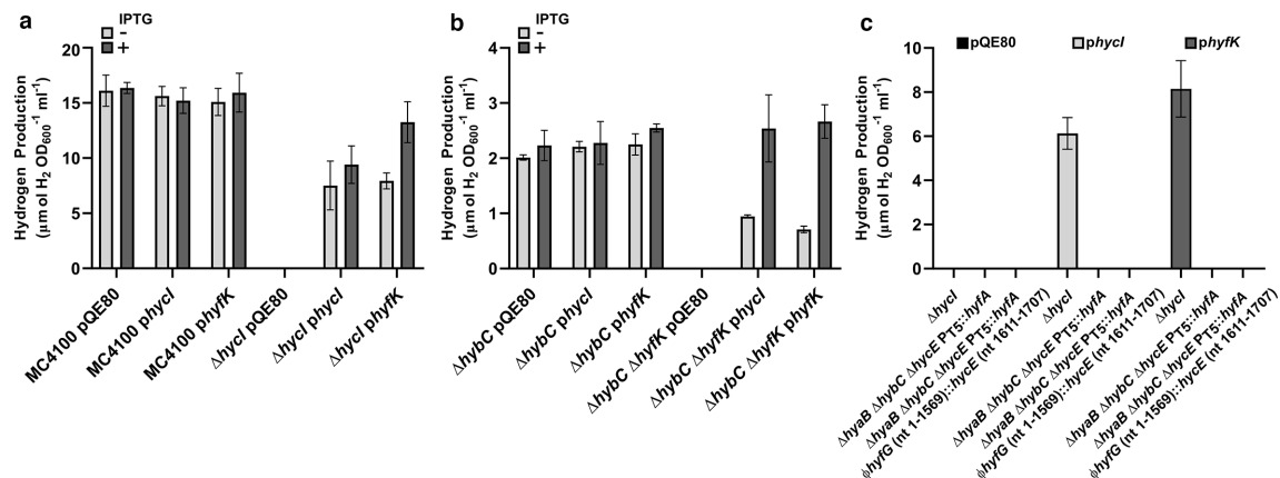
Fig. 2. P. atrosepticum HyfK can activate E. coli Hyd-3, and E. coli HycI can activate P. atrosepticum Hyd-4. (a) E. coli strains MC4100 (FHL-1 + ) and MGE1dI ( \Delta hycI ) were transformed separately with plasmids harbouring hycI Ec , hyfK Pa or a vector control (pQE80). Strains were grown anaerobically in LB medium supplemented with 0.2% (w/v) formate, ampicillin and 1 mM IPTG where indicated (+) for 24 h at 37 °C. (b) P. atrosepticum strains PH002 ( \Delta hycB , FHL-2 + ) and PH006 ( \Delta hycB , \Delta hyfK ) were transformed with plasmids containing hycI Ec , hyfK Pa or pQE80. Strains were grown anaerobically in low-salt LB (LSLB) medium supplemented with ampicillin and 1 mM IPTG where indicated (+) for 48 h at 24 °C. (c) E. coli strains MGE1dI ( \Delta hycI ), FTE003 ( \Delta hyaB , \Delta hycB , \Delta hycE , P T5 :: hyfA ) and FTE004 ( \Delta hyaB , \Delta hycB , \Delta hycE , P T5 :: hyfA , \phi hyfG:: hycE ) were transformed with plasmids containing hycI Ec , hyfK Pa or a vector control (pQE80). Strains were grown anaerobically in LB medium supplemented with 0.8% (w/v) glucose, ampicillin and 1 mM IPTG for 16 h at 37 °C. In all cases, H 2 headspace samples were extracted and analysed by gas chromatography (Shimadzu GC2014 using a 5A molecular packed column with thermal conductivity detection). Data was normalized by OD 600 and culture volume. Error bars represent SD ( n =3).
