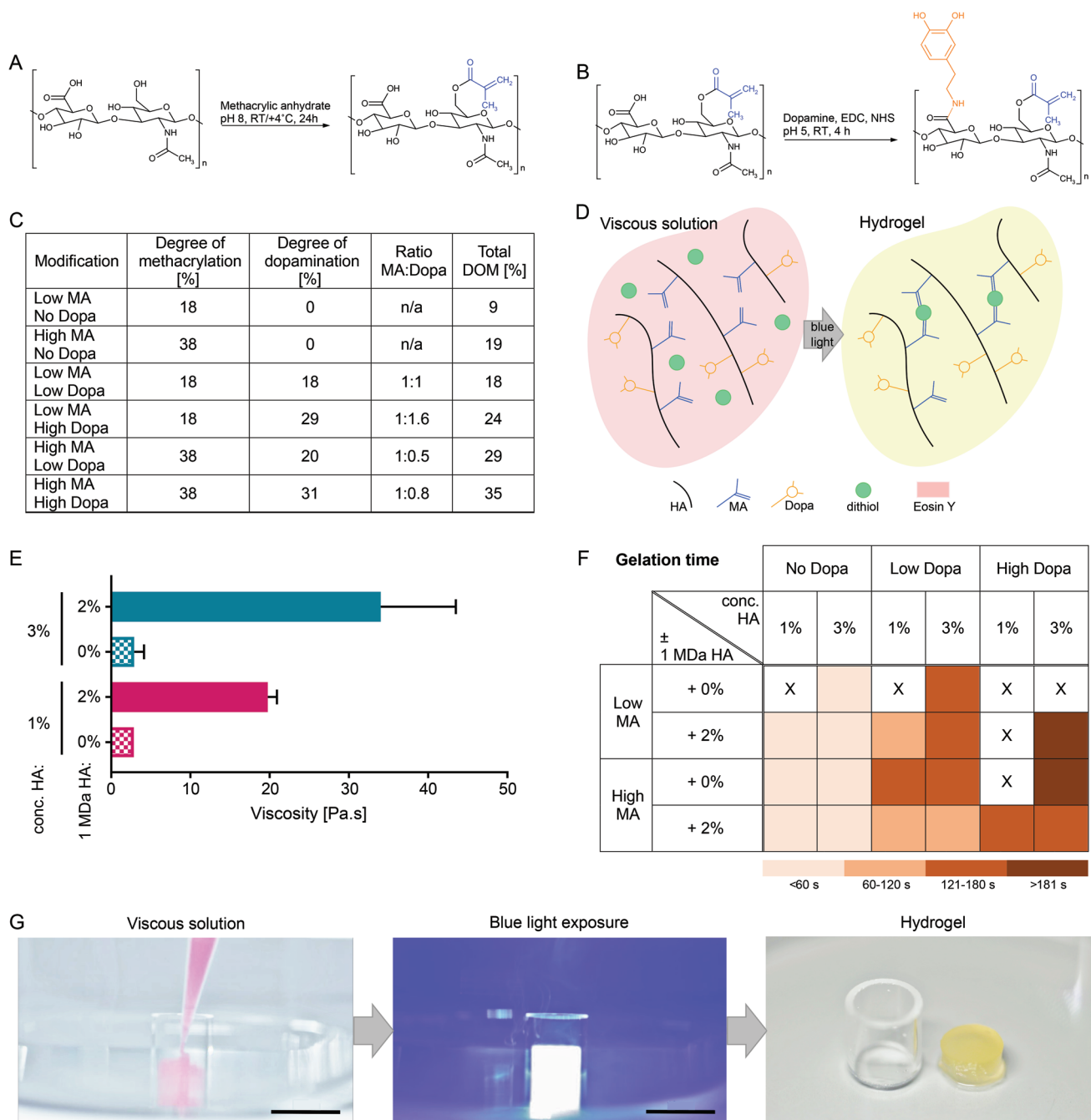
Figure 1. Monomer synthesis and hydrogel formation. A) Synthesis of MA-HA through reaction of HA with methacrylic anhydride; B) Synthesis of MA-HA-Dopa by coupling MA-HA with dopamine; C) Quantification of HA methacrylation and dopamination; D) Reaction schematic demonstrating the formation of hydrogels. Upon blue light exposure, Eosin Y deprotonates di-thiol PEG, allowing it to react with methacrylate moieties on HA leading to a formation of kinetic chains. This process reduces Eosin Y to a colorless state; E) Viscosity of 1% and 3% (w/v) precursor solutions with and without the addition of 2% (w/v) unmodified 1 MDa HA. Plot shows means and standard deviations, n = 3 ; F) Gelation times for different hydrogel compositions. Gelation times were grouped so that light color indicates fast gelation and darker colors show slower gelation; G) Images showing in aqua application of viscous solution and gelation (see also Movie S1 in the Supporting Information), Scale bar = 10 mm.
