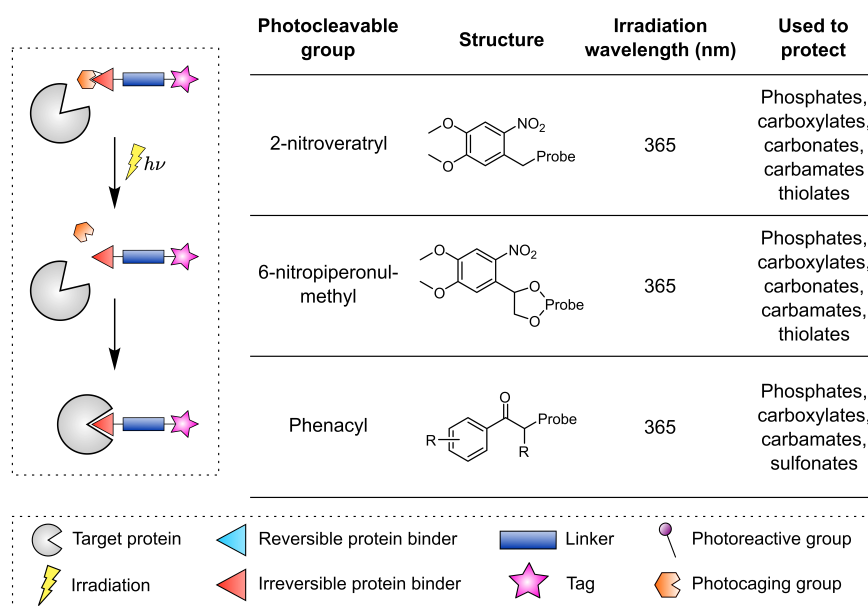
Figure 2. Mechanisms of photoreactive and photocaged probes. A. Photoreactive probes incorporate a reversible protein binder and a photoreactive group which, on irradiation with suitable wavelengths of UV light, form a highly reactive radical which irreversibly binds the protein of interest facilitating the downstream workflow of ABPP. Photocaged probes includes a light-sensitive protecting group on the electrophilic warhead which, on irradiation with UV light, is removed, exposing the warhead which can bind the protein of interest. B. Examples of commonly used photoreactive groups, the wavelength of UV light required to form the reactive radical, and the radical formed [18,59,68]. C. Examples of potential photo caging moieties, including wavelength required for cleavage and groups they can be used to protect, demonstrating the potential breadth of use [69,70].
