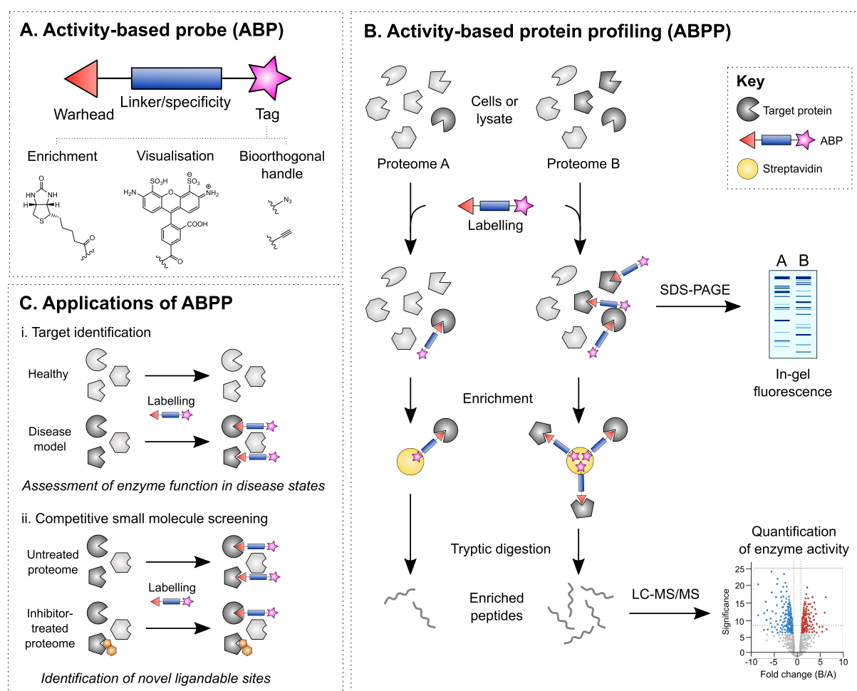
Figure 1. Overview of activity-based protein profiling (ABPP). A. Generic structure of an activity-based probe (ABP). ABPs may be functionalised with affinity tags (e.g. biotin, depicted) and/or fluorophores (e.g. Alexa Fluor 488) for enrichment and visualisation of labelled species, respectively. Latent handles (e.g. azide or alkyne groups) may be incorporated to enable bioorthogonal ligation of tags via copper(I)-catalysed azide-alkyne cycloaddition (CuAAC) [24]. B. General workflow of an ABPP experiment. Typically, proteomes are labelled in cells or in vitro with an ABP directed toward a particular enzyme class or amino acid type. If a fluorophore tag is used, labelled proteins are separated on by SDS-PAGE and directly visualised via fluorescence scanning. By contrast, biotinylated proteins are enriched on a streptavidin-immobilised resin and digested, generating probe-modified peptides for analysis by liquid chromatography-mass spectrometry (LC-MS/MS). Differences
