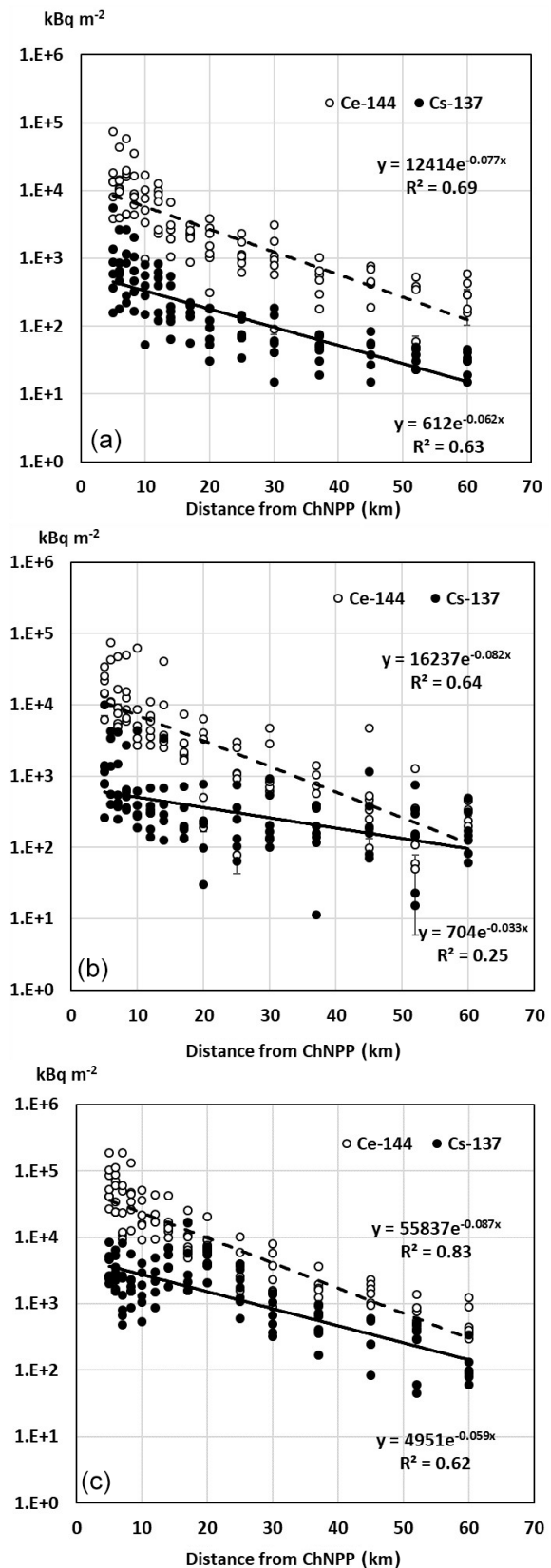
Figure 5. Relationship between fallout density of ^{144}\text{Ce} (1) and ^{137}\text{Cs} (2) and distance from the ChNPP towards the south (a) ( 150\text{--}210^\circ ), the west (b) ( 240\text{--}300^\circ ) and the north (c) ( 330\text{--}30^\circ ).
