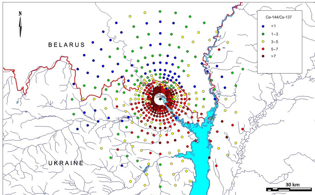
Figure 6. ^{144}\text{Ce} / ^{137}\text{Cs} ratio within the 60 km zone around the ChNPP decay corrected to 6 May 1986.
