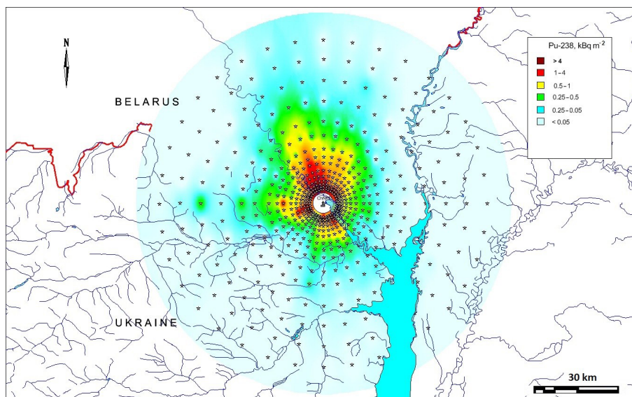
Figure 8. The fallout density of ^{238}\text{Pu} ( \text{kBq m}^{-2} ) corrected to 6 May 1986; estimated from measurements of ^{144}\text{Ce} in the soil and estimated activity concentrations in the fuel of the ChNPP reactor number four (note that no data were available for less than 5 km from ChNPP and no interpolation for this area has been attempted).
