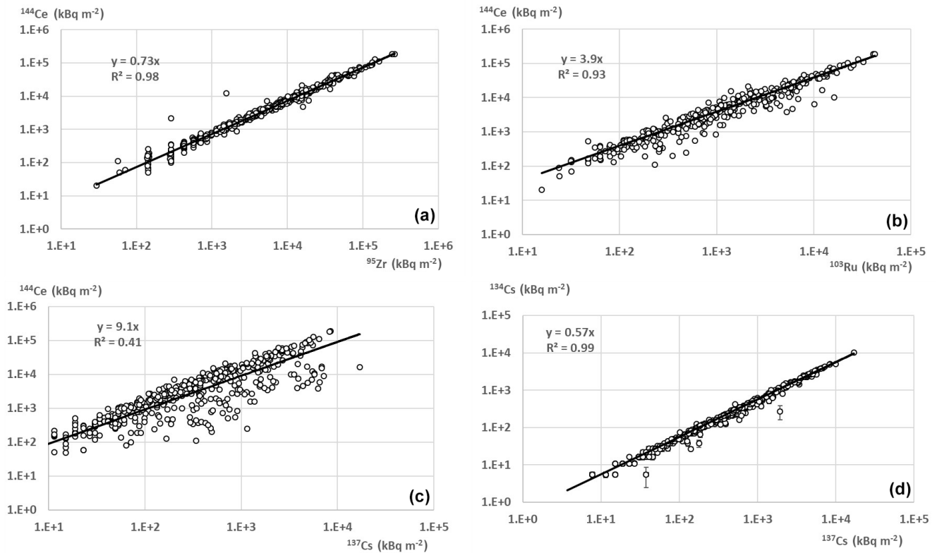
Figure 7. Correlation between deposition densities of different radionuclides decay corrected to 6 May 1986.
