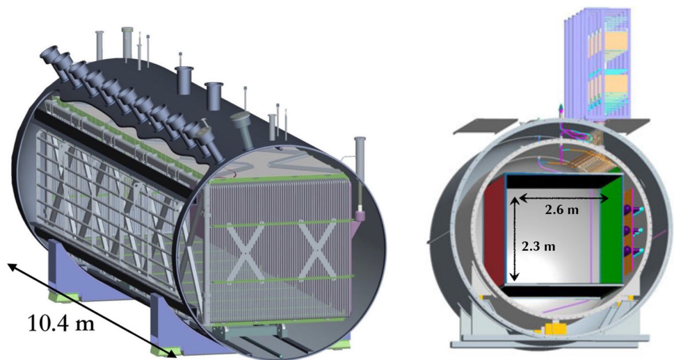
Fig. 1 A schematic view of the MicroBooNE detector. The three wire planes, shown on the right side of the cylindrical cryostat in the right-hand image, contain vertical wires and wires \pm 60^\circ to the vertical. The wire planes are the anode
