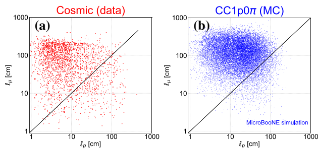
Fig. 5 The distributions of the segmented length of the track labeled as the muon candidate, l_\mu , vs. the track labeled as the proton candidate, l_p , after the application of the cuts on dE/dx and matched PMT flash in MicroBooNE in: a cosmic data, and b simulated CC1p0 \pi events
