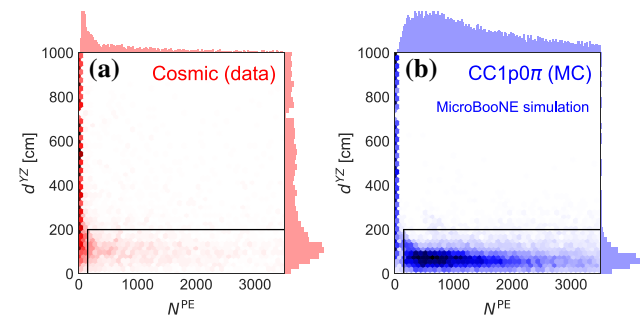
Fig. 4 The distribution of the two-dimensional distance of the reconstructed vertex to the associated flash, vs. the number of photoelectrons (PE) recorded in the flash in: a cosmic data, and b simulated CC1 p0\pi events. Also shown are the one-dimensional projections of the distributions
