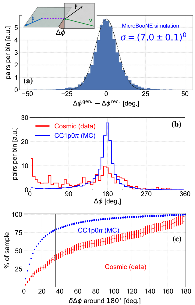
Fig. 9 a The difference between the reconstructed and generated (truth level) \Delta\phi for CC1p0 \pi events in MicroBooNE simulation. A fit for a Gaussian distribution function around the peak is shown in the figure, as well as the width \sigma of the best-fit result. The illustration in the insert shows the definition of the angle. b The distributions of the reconstructed \Delta\phi between the candidate \mu and p candidates after all previous criteria were applied. c The effect of a symmetric selection around \Delta\phi = 180^\circ as a function of the selection criterion
