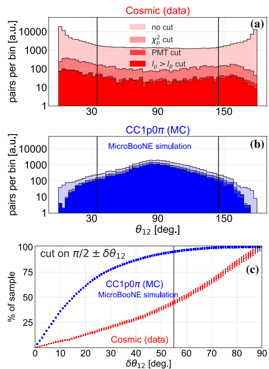
Fig. 6 The distribution of \theta_{12} , in MicroBooNE, for a CR background data, and b CC1p0 \pi simulated signal. A cut of \delta\theta_{12} = |\theta_{12} - 90^\circ| \leq 55^\circ , to suppress background contributions is depicted in the figure. c The impact of a cut on \delta\theta_{12} on the number of simulated signal CC1p0 \pi events lost and the number of CR background events rejected
