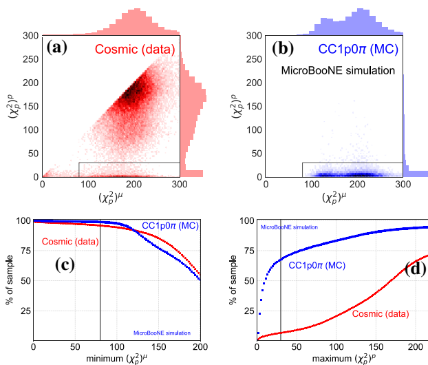
Fig. 3 The distribution of \chi_p^2 of the proton vs. the muon candidate for two identified tracks in a close-proximity pair in MicroBooNE, for a cosmic data and b CC1 p0\pi simulated signal. The proton candidate is labeled as the track with the smaller \chi_p^2 . Also shown are the one-dimensional projections of the distributions. A cut of 80 < (\chi_p^2)^\mu and (\chi_p^2)^p < 30 to suppress CR background contribution is depicted in the figure. c The impact of a cut on (\chi_p^2)^\mu on the number of simulated signal CC1 p0\pi events lost and the number of CR background events rejected. d The impact of a cut on (\chi_p^2)^p on the number of simulated CC1 p0\pi events lost and CR background events rejected
