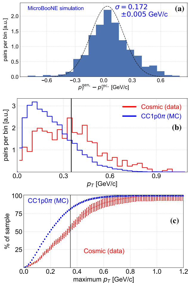
Fig. 10 a The difference between the reconstructed and generated (truth-level) p_T , for simulated CC1 p0\pi signal events. A fit for a Gaussian distribution function around the peak is depicted in the figure, as well as the width \sigma of the best-fit result. b The distributions of the reconstructed p_T between the two tracks, after the application of the detection selection criteria. c The effect of a selection criterion on the maximal reconstructed p_T
