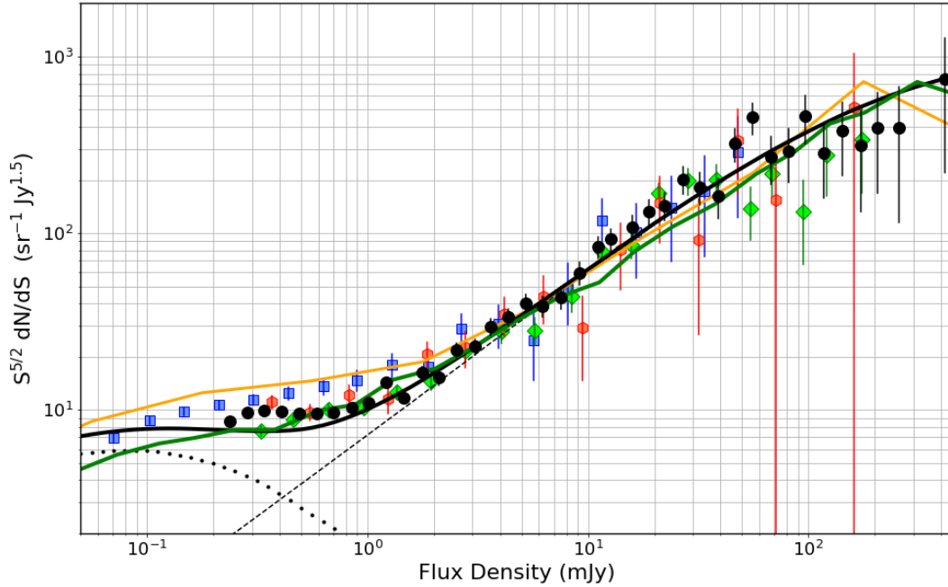
Figure 7. Radio source counts at 610 MHz. Counts from this work are shown as filled black circles. Red hexagons are counts from Bondi et al. (2007), and green diamonds are from Garn et al. (2008). The blue squares are the recent results of very deep GMRT imaging by Ocran et al. (2020). For comparison, the solid lines show model predictions for 610 MHz counts from Wilman et al. (2008) (green), Massardi et al. (2010) (black), and Bonaldi et al. (2019) (orange). The dotted and short dashed lines show indicative model counts for starburst galaxies and AGN from Massardi et al. (2010).
