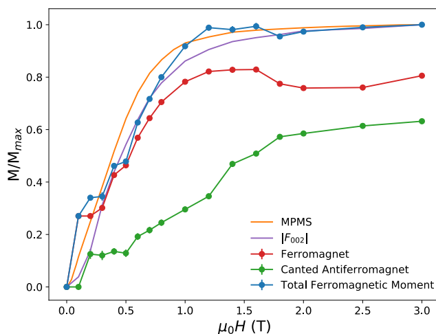
Figure 10. Evolution of the ordered magnetic moments associated with the ferromagnetic phases of TbODCO_3 with respect to applied field. Shown in blue is the total ordered ferromagnetic moment as determined by Rietveld refinement of the diffraction pattern from neutron diffraction data. Shown in orange is the magnetic moment as determined by the MPMS at 2 K, and purple is the structure factor of the ferromagnetic (002) reflection.
