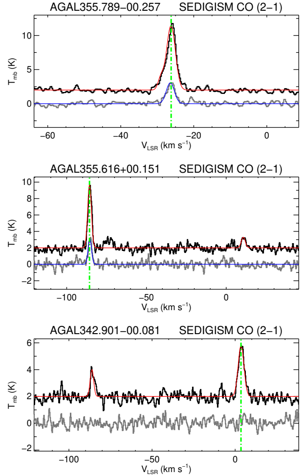
Figure 3. Examples of the 13 CO (black line) and C 18 O (grey) spectra extracted towards three dense clumps identified from the ATLASGAL survey; the former is offset by 2 K from zero intensity. The results of the automatic Gaussian fitting are overlaid in red and blue and the velocity assigned to the clump is indicated by the green vertical dash-dotted line.
