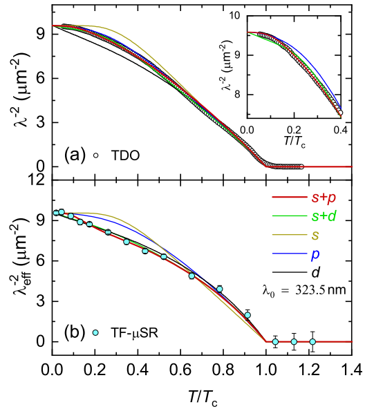
FIG. 7. Temperature dependence of the superfluid density of \text{CaPtAs} , derived from measurements of the magnetic penetration depth using the (a) tunnel-diode oscillator based method, and (b) transverse field \mu\text{SR} . In both cases the superfluid density is best described by a two-gap s+p model, which has one fully open and one nodal gap. Reproduced with permission from Ref. 117. Copyright 2020 by the American Physical Society.
