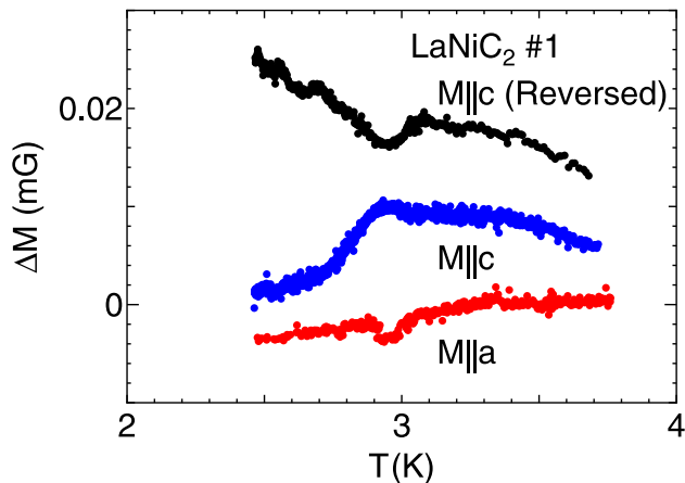
FIG. 3. Temperature dependence of the magnetization change \Delta M(T) of \text{LaNiC}_2 measured upon cooling below T_c in zero-field, with respect to the data at 3.5 K. A clear increase in \Delta M(T) is observed below T_c , while when the sample direction is reversed, there is also a sign change of \Delta M(T) , suggesting the spontaneous occurrence of a bulk magnetization. Reproduced with permission from Ref. 34. Copyright 2015 by the Physical Society of Japan.
