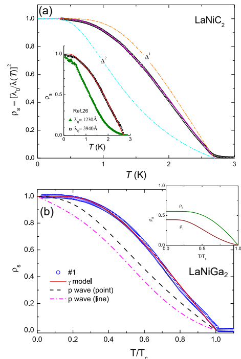
FIG. 4. (a) Temperature dependence of the normalized superfluid density, derived from \Delta\lambda(T) measured using the tunnel-diode oscillator based technique for (a) \text{LaNiC}_2 , and (b) \text{LaNiGa}_2 . The solid lines in both panels show the results from fitting using nodeless two-gap models. Panel (a) is reproduced from Ref. 112, available under a Creative Commons Attribution 3.0 Unported (CC-BY) license. (b) is reproduced with permission from Ref. 14. Copyright 2016 by the American Physical Society.
