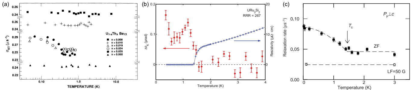
FIG. 1. (a) Temperature dependence of the Gaussian relaxation rate obtained from zero-field \mu SR measurements of U_{1-x}Th_xBe_{13} for different dopings. For stoichiometric UBe_{13} , no change is observed below T_c , but for 2-4% Th-doping, an increase in the relaxation rate is observed below the emergent second superconducting transition. Reproduced with permission from Ref. 32. Copyright 1990 by the American Physical Society. (b) Temperature dependence of the Kerr angle and resistivity of URu_2Si_2 . The increase of the Kerr angle indicates the breaking of time reversal symmetry, and it can be seen that this onsets at the superconducting transition. Reproduced with permission from Ref. 23. Copyright 2015 by the American Physical Society. (c) Temperature dependence of the Lorentzian relaxation rate ( \lambda_{ZF} in Eq. 4) obtained from zero-field \mu SR on Sr_2RuO_4 , with the initial muon spin polarized perpendicular to the c -axis. This quantity shows an increase below T_c indicating TRS breaking, while this effect is destroyed by a longitudinal field of 50 mT. Reproduced with permission from Macmillan Publishers Ltd: Nature 33 , copyright 1998.
