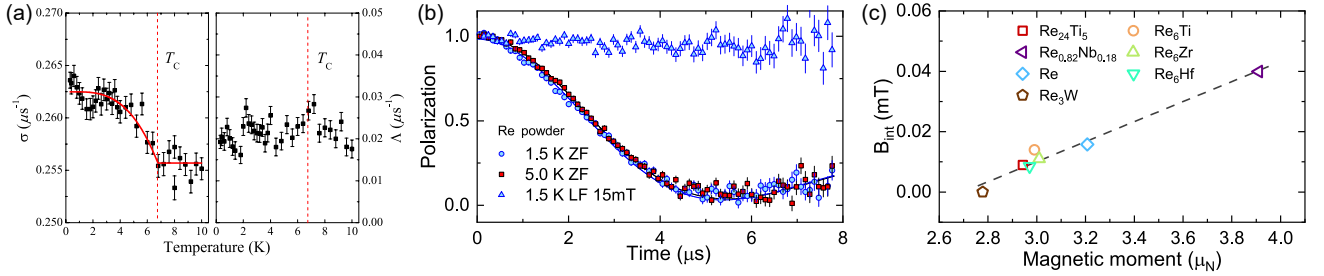
FIG. 5. (a) Temperature dependence of the Lorentzian and Gaussian relaxation rates obtained from zero-field \mu\text{SR} measurements of \text{Re}_6\text{Zr} , where the latter shows a clear increase below T_c indicating TRS breaking. Reproduced from Ref. 114, available under a Creative Commons Attribution 3.0 License. (b) \mu\text{SR} time spectra of elemental Re measured in zero-field above and below T_c , and in a longitudinal field of 15 mT in the superconducting state. The more rapid depolarization below T_c indicates the presence of TRS breaking of elemental Re, and as shown in the inset this onsets below T_c . (c) Plot of the internal field estimated from the increase of \sigma_{ZF} below T_c as a function of the nuclear moment calculated from the nuclear moments of the constituent elements and their relative fractions. A clear positive correlation is observed between the two quantities. Both (b) and (c) are reproduced with permission from Ref. 115. Copyright 2018 by the American Physical Society.
