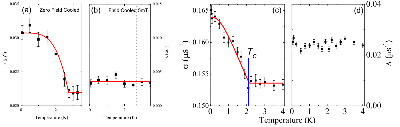
FIG. 2. Lorentzian relaxation rate \lambda_{ZF} obtained from fitting \mu SR spectra of LaNiC 2 in (a) zero-field, and (b) a longitudinal field of 5 mT. In zero-field there is a clear increase of \lambda_{ZF} correlated with T_c , which disappears in the longitudinal field. Reproduced with permission Ref. 11. Copyright 2009 by the American Physical Society. From the analysis of the zero-field \mu SR of LaNiGa 2 , the temperature dependence of the (c) the Gaussian relaxation rate \sigma_{ZF} , and (d) the Lorentzian relaxation rate \Lambda are displayed. In this case \sigma_{ZF} shows a clear increase below T_c , while \Lambda remains unchanged. Reproduced with permission Ref. 13. Copyright 2012 by the American Physical Society.
