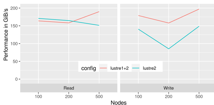
Figure 9. Lustrre performance for 100, 200, and 500 nodes
