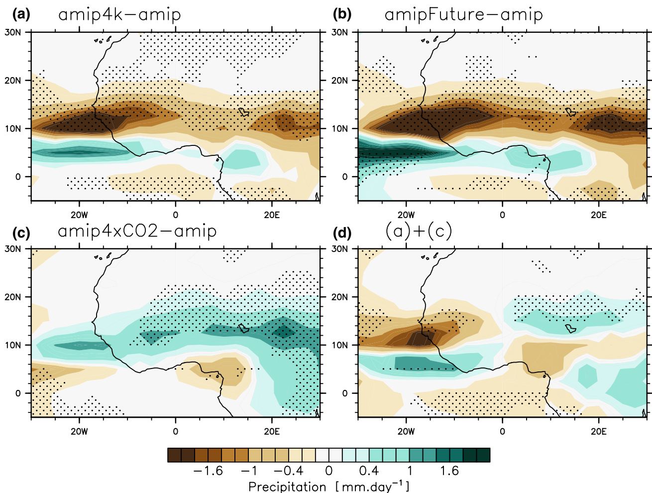
Fig. 8 Difference in July–September ensemble mean precipitation ( \text{mm}\cdot\text{day}^{-1} ) between a the CMIP5 amip4K and amip, b amip-Future and amip, c amip4xCO2 and amip simulations. d Sum of the
