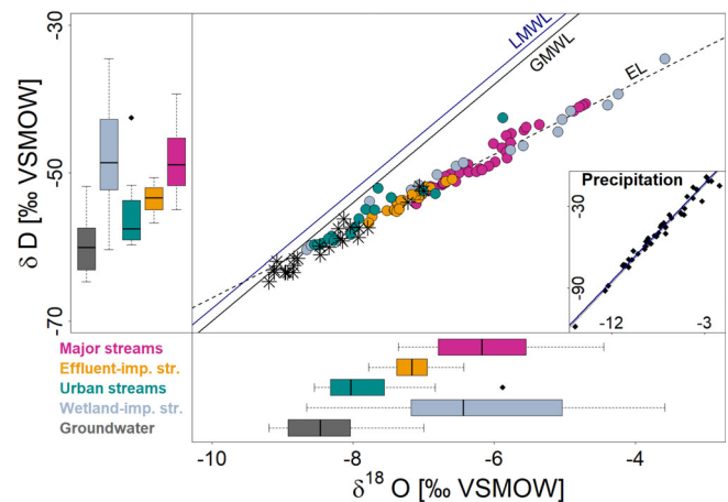
FIGURE 5 Dual isotope plot (centre) and box plots (left, bottom) showing the isotopic composition of the different seasonal surface water types and groundwater during the four seasonal sampling campaigns. global meteoric water line and amount-weighted local meteoric water line from precipitation samples in Berlin-Friedrichshagen (inset) are given for reference
