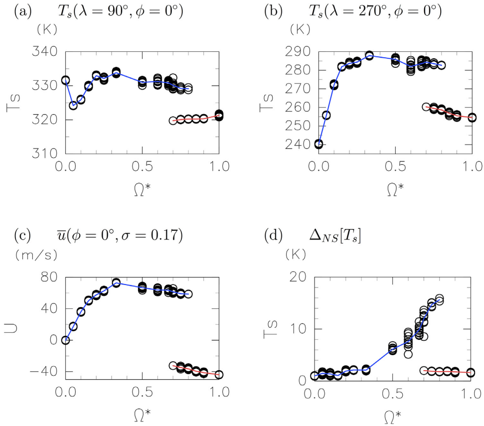
Fig. 4. \Omega^* dependences of (a) surface temperature [K] at the subsolar point, (b) surface temperature [K] at the antipolar point, (c) zonal mean equatorial zonal wind [ \text{m s}^{-1} ] at \sigma = 0.17 , and (d) degree of north-south asymmetry of surface temperature defined by Eq. 2 in the text [K]. The values are temporal averages between day 1000 and day 2000. All 10 runs for each \Omega^* case are plotted. Red and blue lines are ensemble averages for the small- \Omega^* and the large- \Omega^* branches, respectively. (For interpretation of the references to colour in this figure legend, the reader is referred to the web version of this article.)
