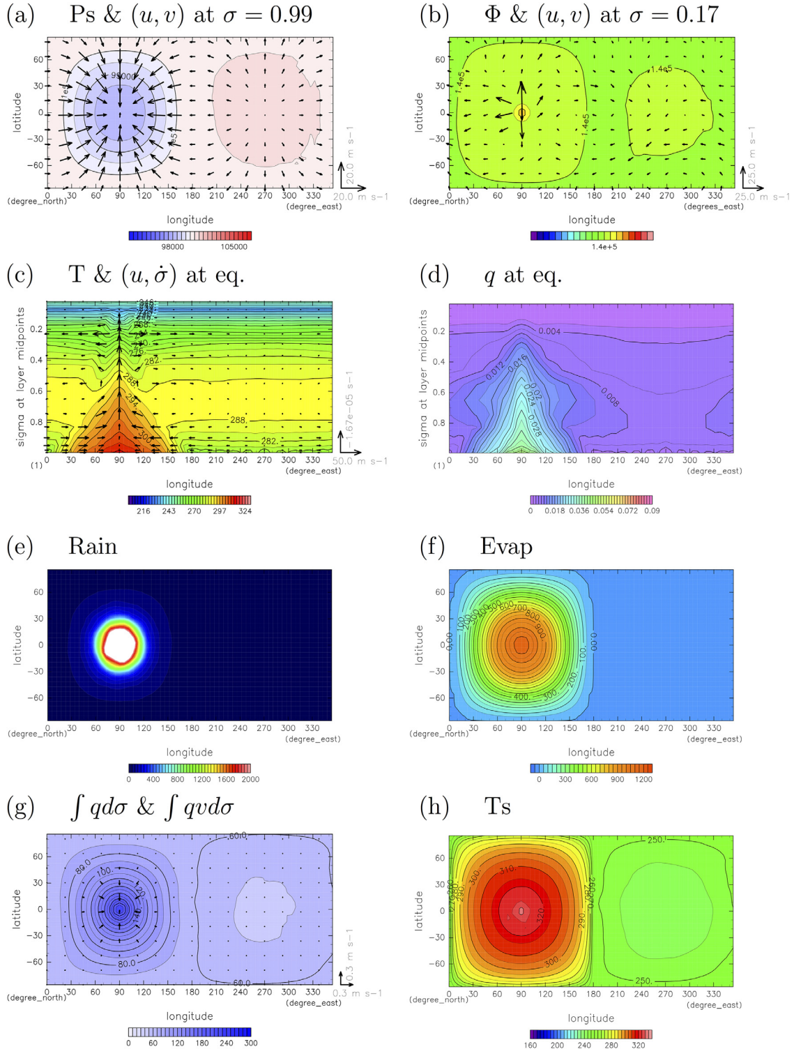
Fig. 5. Day 1000 to day 2000 temporal mean fields for case \Omega_{20.0} . (a) Surface pressure (color shading) [Pa] and horizontal wind vectors [ \text{m s}^{-1} ] at the lowest level. Contour interval of surface pressure is 5 \times 10^2 Pa, and the unit vectors of zonal and meridional wind are 20 \text{ m s}^{-1} . (b) Horizontal wind vector [ \text{m s}^{-1} ] and geopotential [ \text{J kg}^{-1} ] at \sigma = 0.17 . Unit vector indicates 25 \text{ m s}^{-1} . Contour interval of geopotential is 500 \text{ J kg}^{-1} . (c) Vertical wind -\sigma [ \text{s}^{-1} ] and zonal wind [ \text{m s}^{-1} ] (vector), and temperature [K] (color) in the equatorial vertical section. Unit vectors of vertical wind and zonal wind are 1.67 \times 10^{-5} \text{ s}^{-1} and 50 \text{ m s}^{-1} , respectively. Contour interval of temperature is 5 \text{ K} . (d) Specific humidity at the equator. Contour interval is 2 \times 10^{-3} . (e) Condensation heating [ \text{W m}^{-2} ]. Color interval is 50 \text{ W m}^{-2} . White area represents heating over 2000 \text{ W m}^{-2} . (f) Horizontal distribution of surface evaporation [ \text{W m}^{-2} ]. Color interval is 50 \text{ W m}^{-2} . (g) Vertically integrated water vapor flux [ \text{m s}^{-1} ] and vertically integrated water vapor mass [ \text{kg m}^{-2} ]. Unit vector is 0.3 \text{ m s}^{-1} . Contour interval is 10 \text{ kg m}^{-2} . (h) Surface temperature [K]. Contour interval is 5 \text{ K} . (For interpretation of the references to colour in this figure legend, the reader is referred to the web version of this article.)
