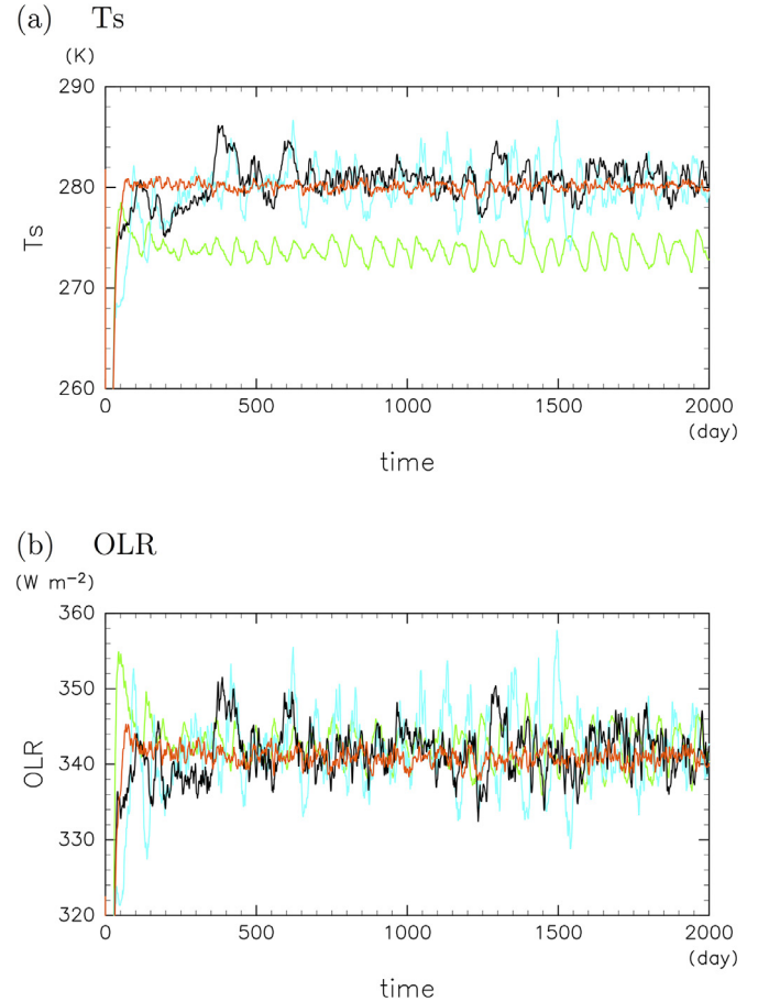
Fig. 2. Time series of global mean quantities. (a) Surface temperature [K] and (b) OLR [ \text{W m}^{-2} ]. Green, light-blue, black, and red lines indicate \Omega 0.0 , \Omega 0.15 , \Omega 0.75 , and \Omega 1.0 , respectively. (For interpretation of the references to colour in this figure legend, the reader is referred to the web version of this article.)
