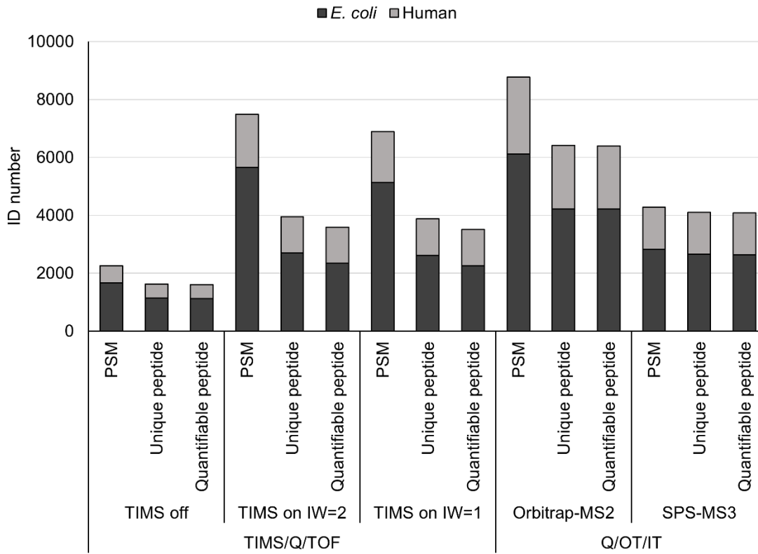
Figure S2. An overview of the identification results. Peptide spectrum match (PSM), unique peptide and quantifiable peptide numbers are shown. E. coli peptides with all the six reporter ions and human peptides with all the three reporter ions were considered as quantifiable peptide. IW: quadrupole isolation window.
