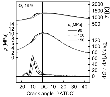
Fig. 6a Heat release rate, in-cylinder pressure, and average in-cylinder temperature as function of crank angle when sub-injection pressure was modified.
