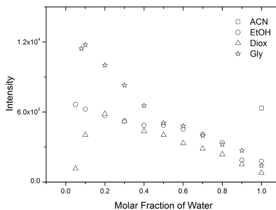
Figure 3. Changes of the fluorescence intensity measured at the maximum of emission for the binary solvent mixtures studied in this work. The excitation wavelength was adjusted at 640 nm. □) acetonitrile; ○) ethanol; Δ) dioxane; *) glycerol.
