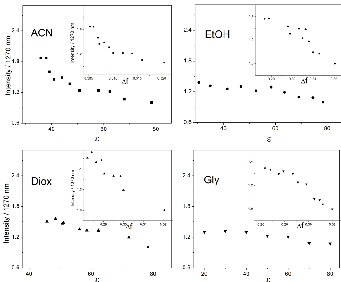
Figure 6. Intensity change of singlet oxygen emission in ACN (acetonitrile), EtOH (ethanol), Gly (glycerol) and Diox (dioxane) as a function of the dielectric constant and solvent polarity parameter, \Delta f (inset). MB concentration of 3.13 \times 10^{-4} \text{ mol L}^{-1} . The excitation wavelength was fitted at 665 nm.
