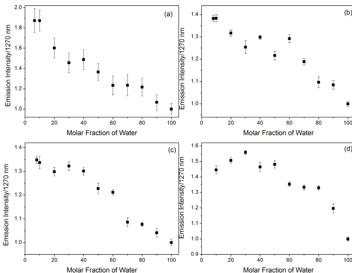
Figure 5. Changes in singlet oxygen emission intensities in (a) acetonitrile, (b) ethanol, (c) glycerol and (d) dioxane as a function of the water content. MB concentration of 3.13 \times 10^{-4} \text{ mol L}^{-1} . The excitation wavelength was fitted at 665 nm.
