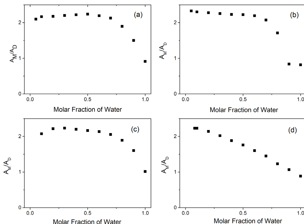
Figure 2. Changes of A_M/A_D ratio ( A_M = monomer absorbance and A_D =dimer absorbance) in different binary solvent mixtures: (a) water/acetonitrile; (b) water/ethanol; (c) water/dioxane and (d) water/glycerol. [\text{MB}] = 3.13 \times 10^{-4} \text{ mol L}^{-1} .
