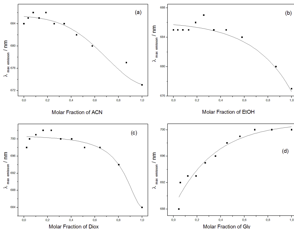
Figure 4. Shift of the emission maximum of MB as a function of the molar fraction of the solvent mixture: a) water/acetonitrile; b) water/ethanol; c) water/dioxane and d) water/glycerol. The excitation wavelength was fitted at 640 nm.
