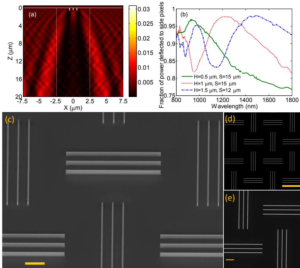
Fig. 3. (a) Simulated power flow for light polarized parallel to length of nanoridges ( y -direction). Wavelength of operation is \lambda=950 nm. There are three nanoridges with widths W=50 nm, heights H=500 nm, center-to-center distance P=550 nm, and lengths L=5 \mu m. After z=14 \mu m majority of power presents in side pixels region. Boundaries of pixels are highlighted by dashed lines. For this simulation, the total transmission, reflection and absorption are 94.5%, 5% and 0.5 % respectively. (b) Fraction of transmitted power that is deflected to side pixels versus wavelength for three different designs. Designs are optimized for center wavelengths close to 1000 nm, 1200 nm and 1500 nm. By deviating from design wavelength, phase difference will no longer takes the value \pi ; therefore, we shift from “destructive interference condition”, and the proportion of input light power that is split (deflected) is reduced. For all simulations, there are three nanoridges with widths W=50 nm, center-to-center distance P=550 nm and lengths L=5 \mu m. Heights of nanoridges and distance from substrate where power is recorded are noted in figure’s caption. (c)-(e) SEMs of fabricated PIXIP device. (c) Tilted-view SEM of PIXIP device, scale bar is 1 \mu m. (d) Top-view SEM of PIXIP device, scale bar is 5 \mu m. (e) Top-view SEM depicting one unit cell of PIXIP device, scale bar is 1 \mu m.
