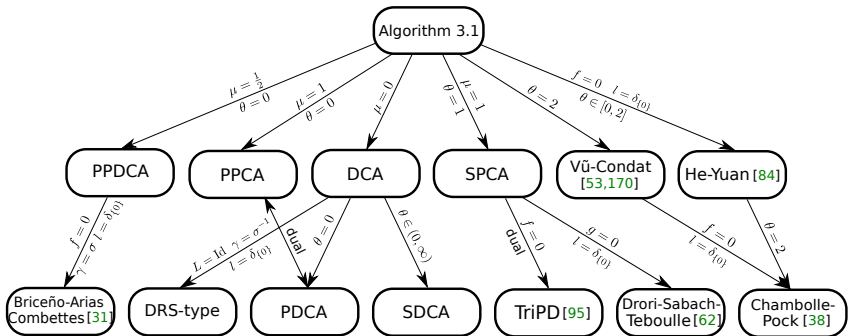
Figure 1.1: Algorithm 3.1 and its special cases
