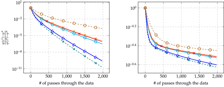
Figure 8.1: Performance comparisons for Algorithms 8.2 and 8.3 for problem (8.39) with different initial points: (left) x^{\text{init}} = 0_n , (right) x^{\text{init}} = 1_n . Algorithm names ending with -\gamma indicate the use of a single stepsize \gamma = \min_i \gamma_i .
