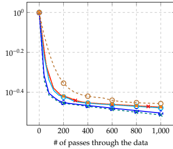
Figure 8.3: Performance comparisons for Algorithms 8.2 and 8.3 for problem (8.40) with different initial points: (left) x^{\text{init}} = 0_n , (right) x^{\text{init}} = 1_n . Algorithm names ending with -\gamma indicate the use of a single stepsize \gamma = \min_i \gamma_i
