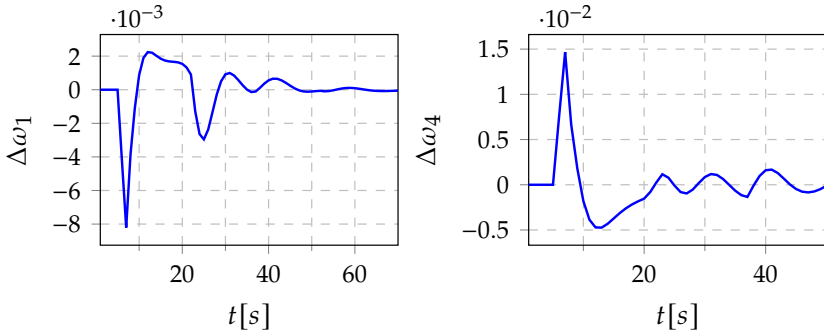
Figure 5.3: Frequency deviation for systems one and four
