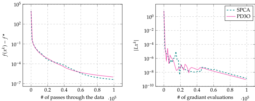
Figure 3.2: Performance comparisons for SPCA and PD30 [180] for classifying a1a dataset
