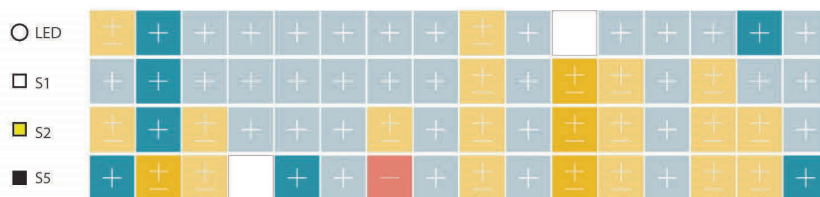
Figure 28. SDG implications of alternative strategies of limited global warming to below 1.5°C. Source: IPCC Special Report on 1.5°C, Rogelj et al. (2018), Figure 2.28.
