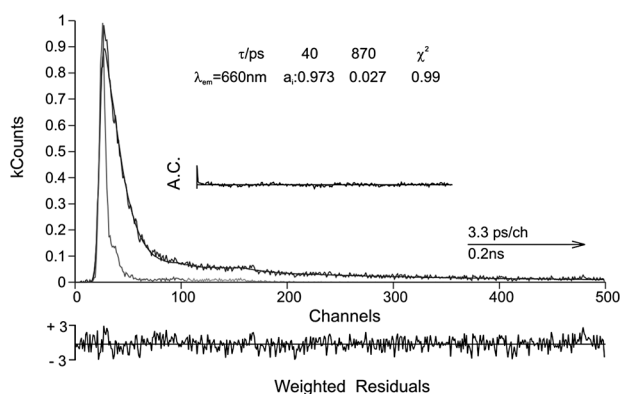
Fig. 3 Fluorescence decay and pulse instrumental response (short pulse) for the indigo polymer in DMF at T = 293 K. Shown as insets are the decay times and pre-exponential factors. Also shown are the weighted residuals, autocorrelation functions (A.C.) and the \chi^2 values for a better judgment of the quality of the fits.
