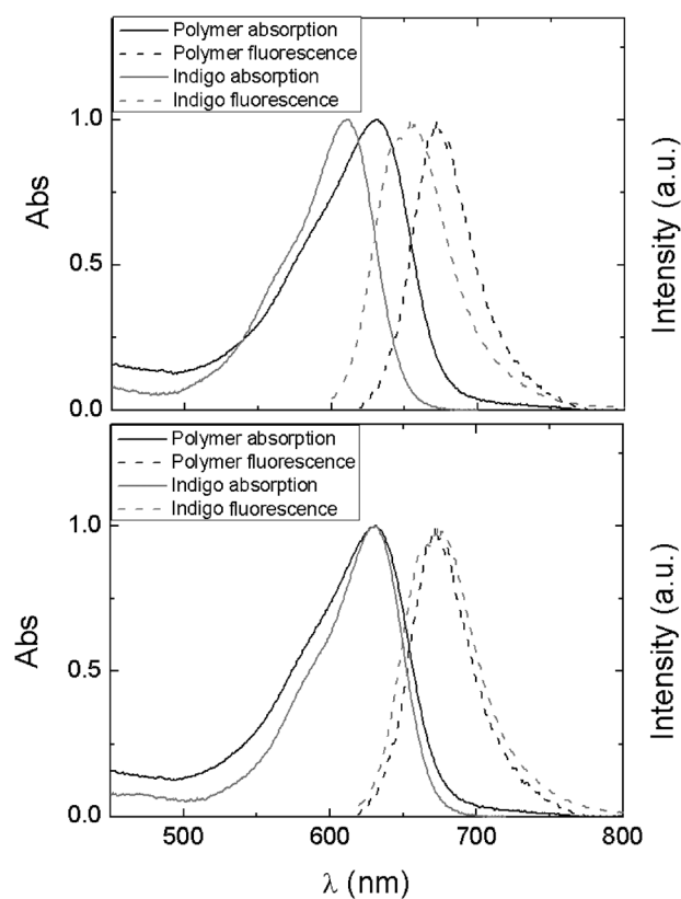
Fig. 2 Absorption and fluorescence spectra for indigo and the indigo polymer in DMF. In the top panel the spectra are normalized at its intensity/abs maxima, whereas in the bottom panel the absorption spectra of indigo and of its polymer are (artificially) set to have the same maxima and the same is valid for the emission spectra, where now the differences in the inhomogeneous broadening can be better visualized.
