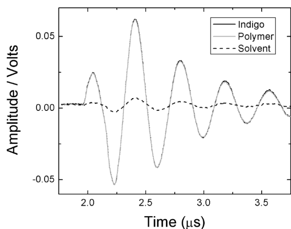
Fig. 5 Example of a typical PAC experiment with the waves for 100% laser intensity: reference wave (indigo, full black line), sample wave (full grey line); sample and reference in DMF (solvent) at 293 K.
