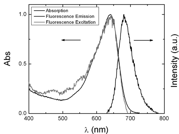
Fig. 1 Absorption and fluorescence emission and excitation spectra of the indigo polymer in DMSO, T = 293 K.
