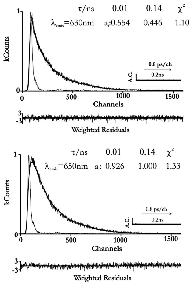
Fig. 4 Fluorescence decay and pulse instrumental response for indigo in DMF, collected at two different emission wavelengths at T = 293 K. Shown as insets are the decay times and pre-exponential factors. Also shown are the weighted residuals, autocorrelation functions (A.C.) and the \chi^2 values for a better judgment of the quality of the fits.
