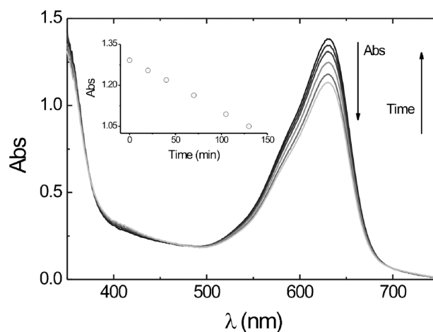
Fig. 6 Polymeric indigo in DMF, irradiated at 335 nm and 293 K, followed by UV-Vis absorption; as the inset shows the plot of the variation in absorbance at 630 nm, for the initial times, from which, compared with indigo under the same experimental conditions, the \phi_R value could be obtained.
