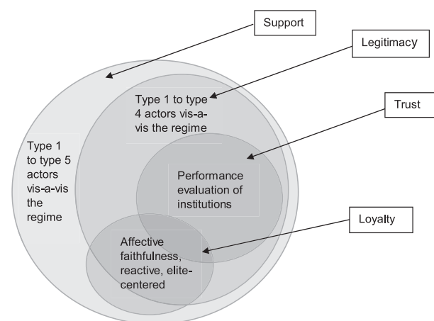
Figure 2 Semantic map
