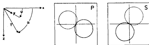
Fig. 17. Single-force radiation patterns. Left: The force is inclined by angle \varphi from the horizontal axis. Right: The single force radiation patterns of P and S waves for \varphi=30^\circ . The solid line denotes positive values, dashed line negative values. \vec{i} denotes the initial direction of the ray
