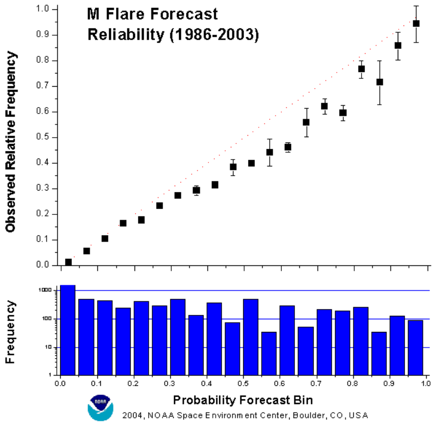
Figure 1.7 – SEC Flare Probability Forecast Verification Plot
