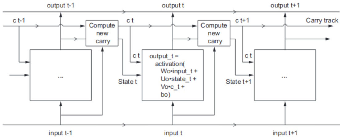
Figure 13: An LSTM architecture [8]
