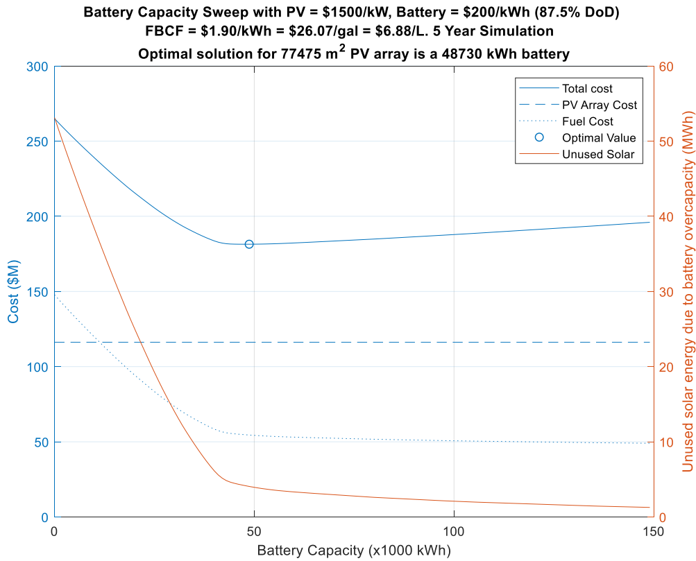
Figure 34. 5-year Li-Ion Optimal Battery Size given PV Area of 77,475 m 2
