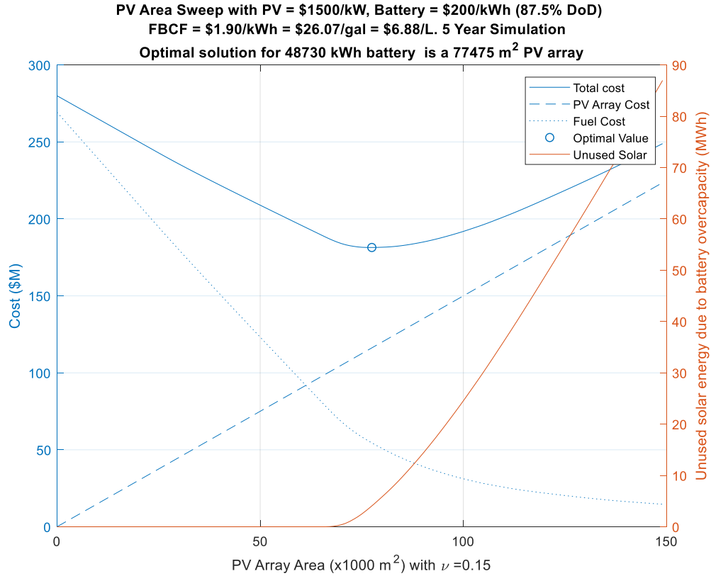
Figure 33. 5-year Li-Ion Optimal PV Area given Battery Size 48,730 kWh
