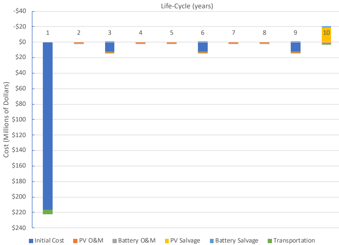
Figure A-6: 10-year Cash Flow Diagram for Lead-Acid with Salvage Values
