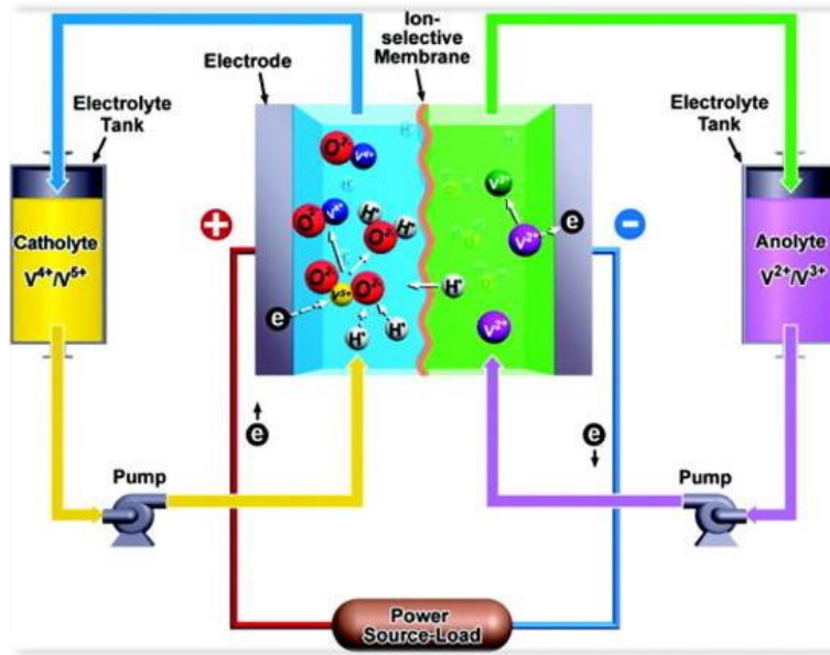
Figure 2. VRFB Diagram [21]
