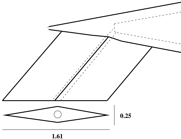
Figure 11: Sting setup [16]
