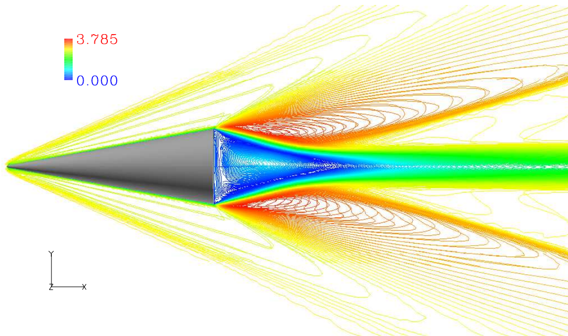
Figure 15: Contours of mach for carrier in free flight, Mach = 2.93
