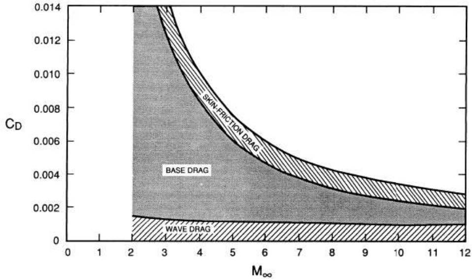
Figure 3: Components of total drag for a cone with a 2.9 degree half-angle [19]
