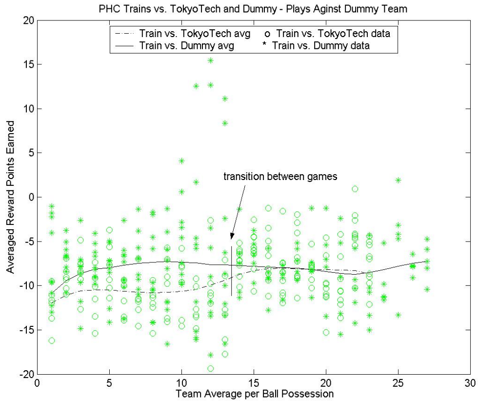
Figure 4.7: PHC with PHC Team Learns vs. TokyoTech and Dummy Team – Plays vs. Dummy Team.
