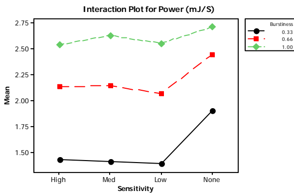
Figure 26 - Mean power for interaction of sensitivity and burstiness
