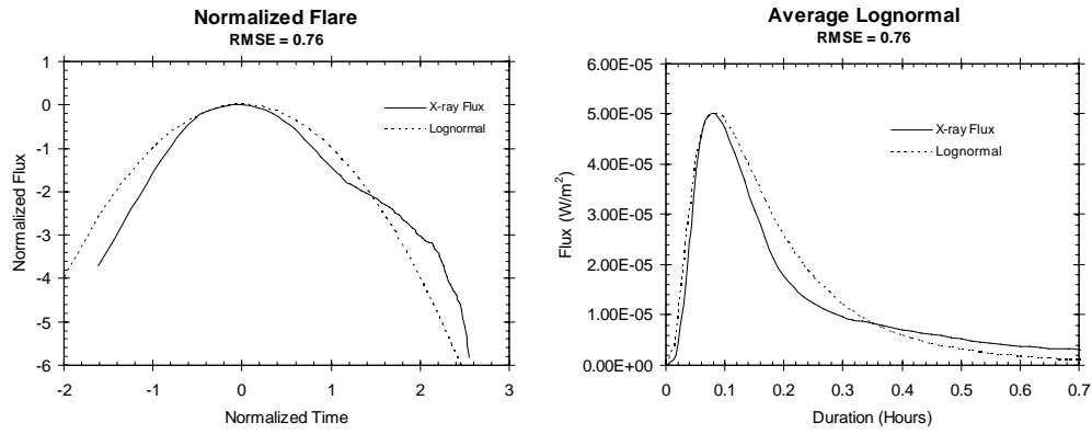
Figure 17. A flare from 26 Jul 2002 with an RMSE that is the same as the average RMSE of 0.76. The left panel shows the normalized flare. The right panel shows the same flare in real time.
