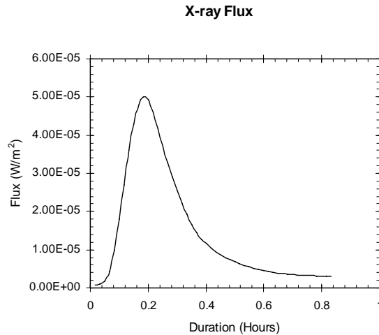
Figure 10. A peak flux of 5 \times 10^{-5} \text{ W/m}^2 gives an M5 classification for this flare from 03 Nov 2004.
