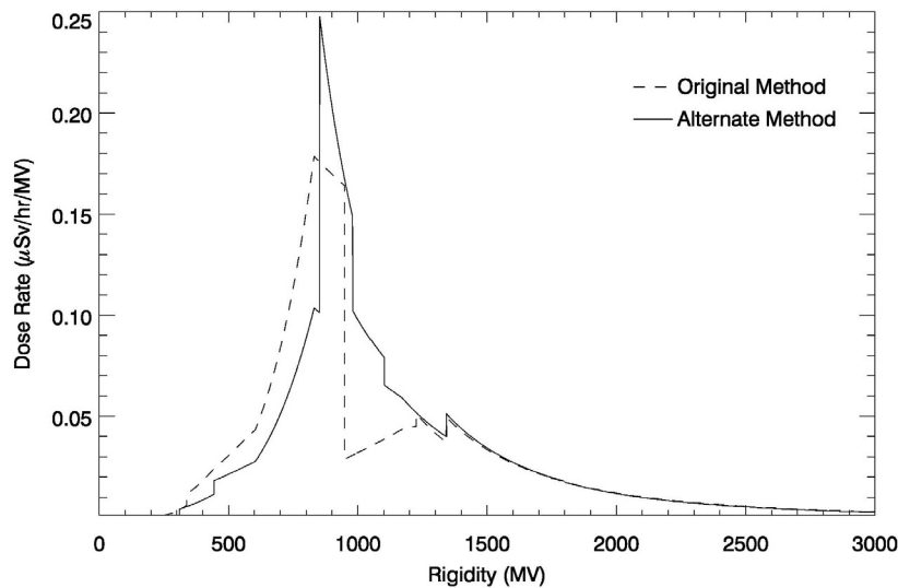
Figure 15: Comparison of the differential effective dose rate as a function of rigidity using the original method and the alternate method. The original method exhibits a troubling discontinuity from 950 to 1225 MV. The alternate method displays a more realistic looking differential dose rate across this range of rigidities.
