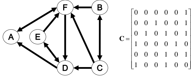
Figure 2.8: Katz Choice Matrix [Katz, 1953, pg. 40]
