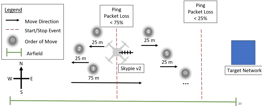
Figure 26: Ping mode's capture process (experiment 2)
