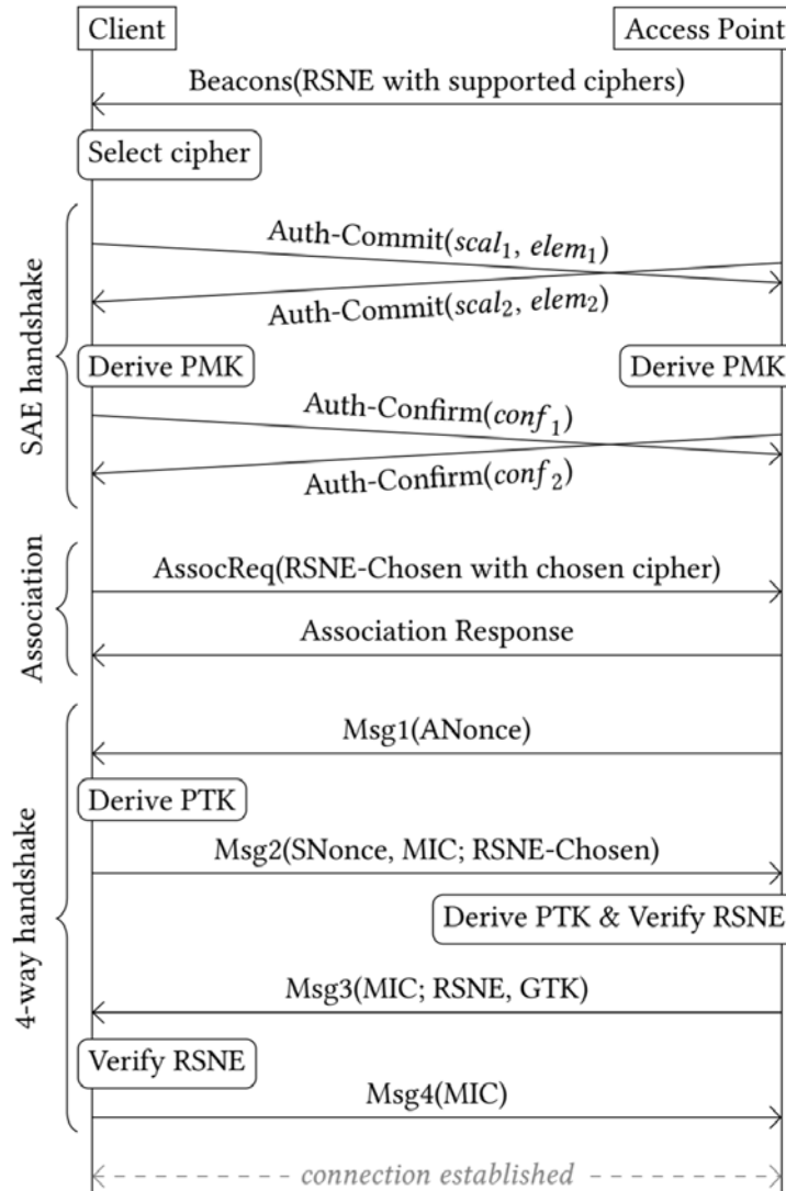
Figure 5: WPA3 authentication [45]
