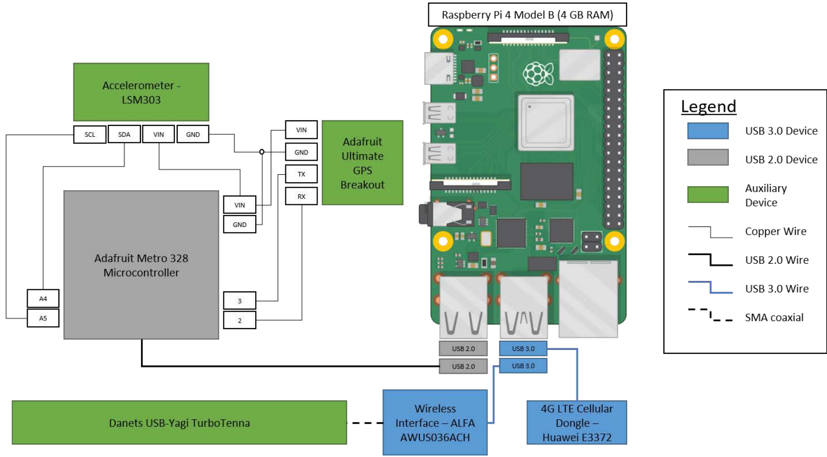
Figure 13: Skypie v2 hardware schematic
