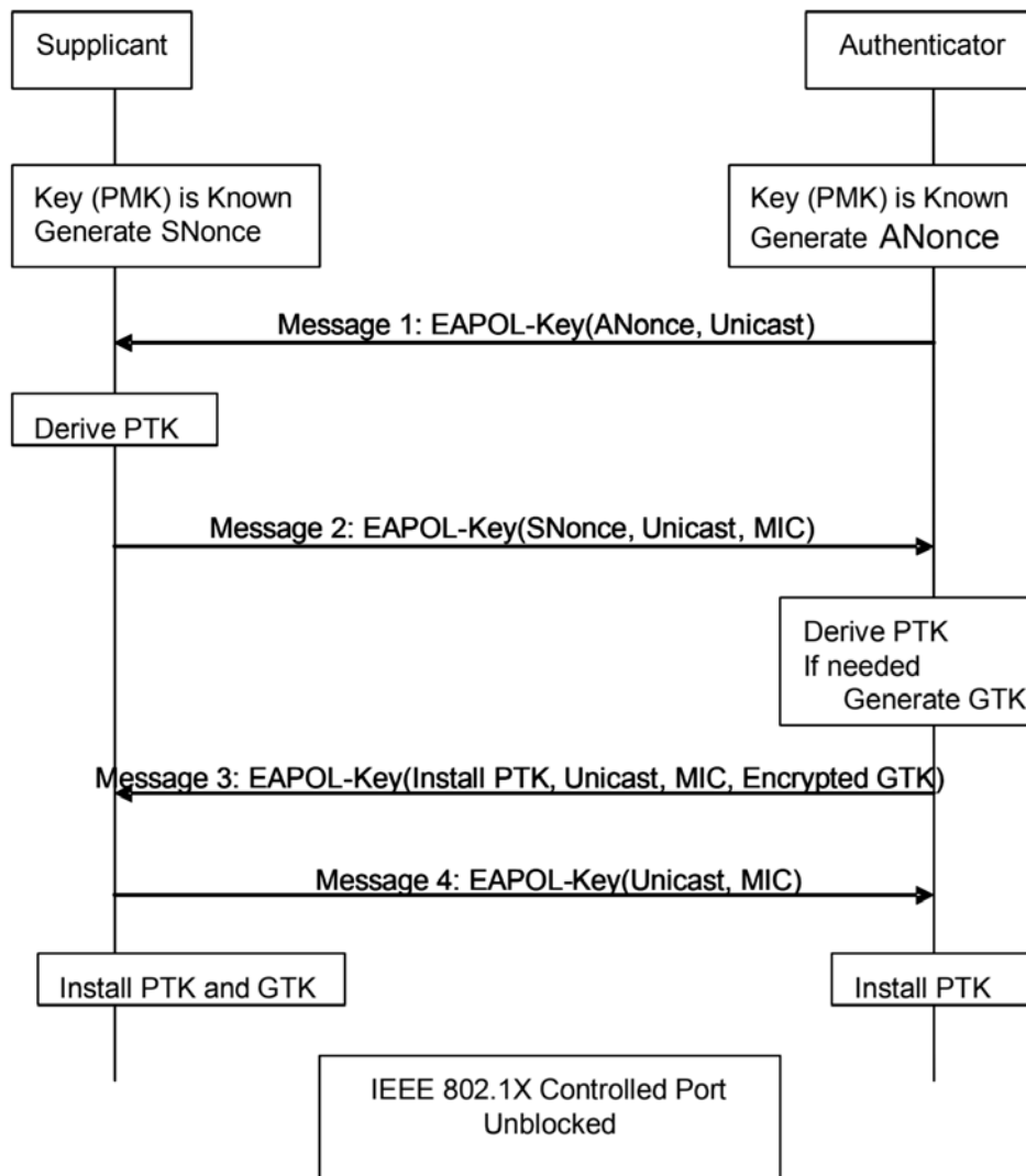
Figure 4: WPA2 four-way handshake [41]
