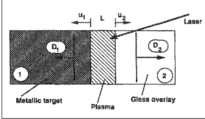
Figure 7: 1D shock propagation from LSP pressure impulse [92]
