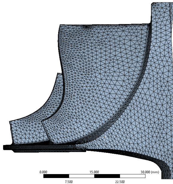
Figure 50. Adaptive Mesh for Stock JetCat P400
