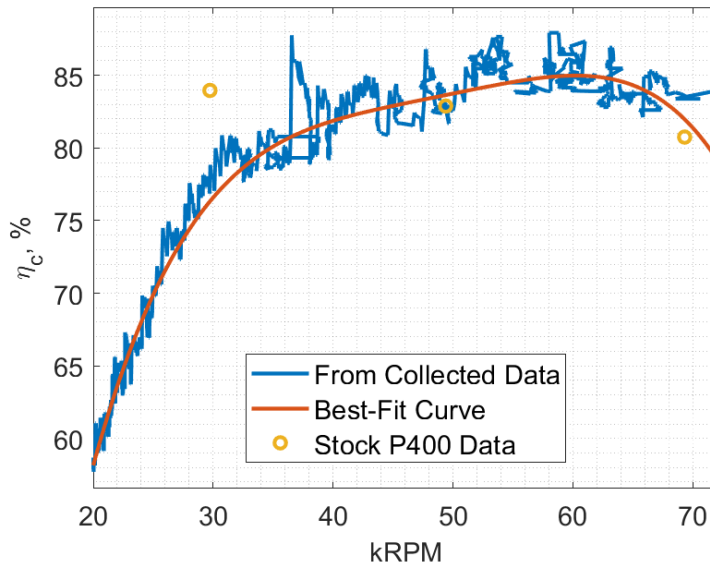
Figure 109. Isentropic Efficiency vs. RPM P400 Compressor, ULTEM 9085 Test.
