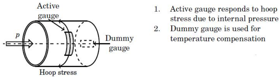
Figure 36. Schematic of a Pressure Tube [60]
