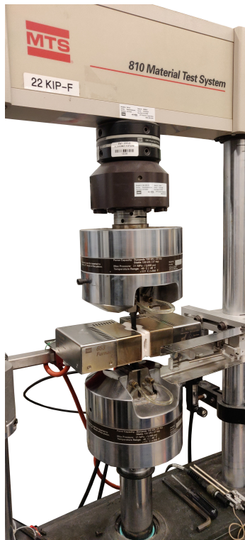
Figure 43. Heated Material Test System with ULTEM 9085 Test Specimen
