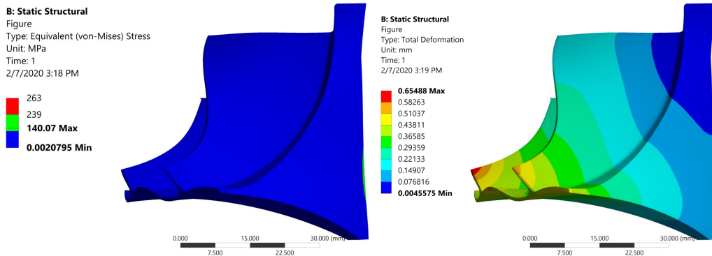
Figure 120. Stresses and Deformation for Modified P400 Compressor, Onyx-Carbon Fiber, 98,000 RPM
