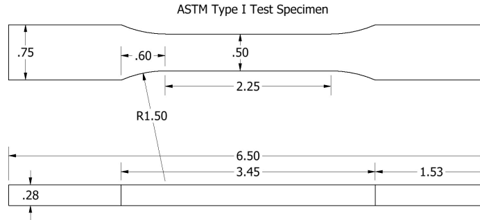
Figure 44. ASTM Type I Tensile Test Specimen
