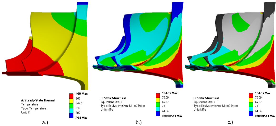
Figure 52. Post-Processing to Account for Temperature-Dependent Ultimate Strength
