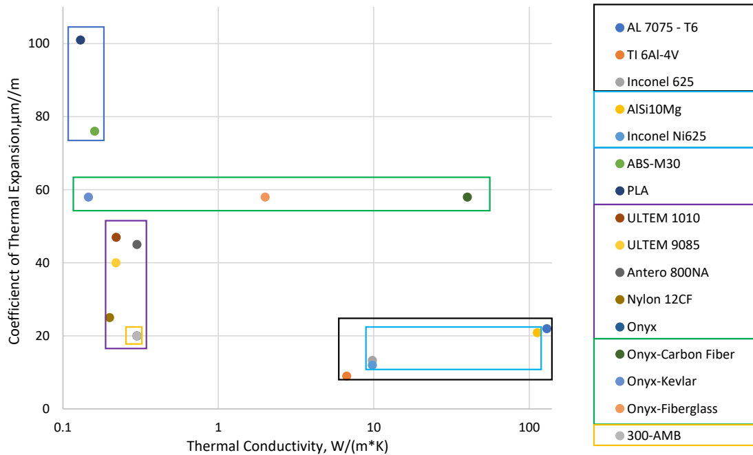
Figure 33. Thermal Conductivity versus Coefficient of Thermal Expansion
