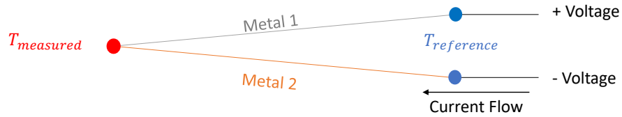
Figure 40. Schematic of a Thermocouple under the Seebeck Effect.
