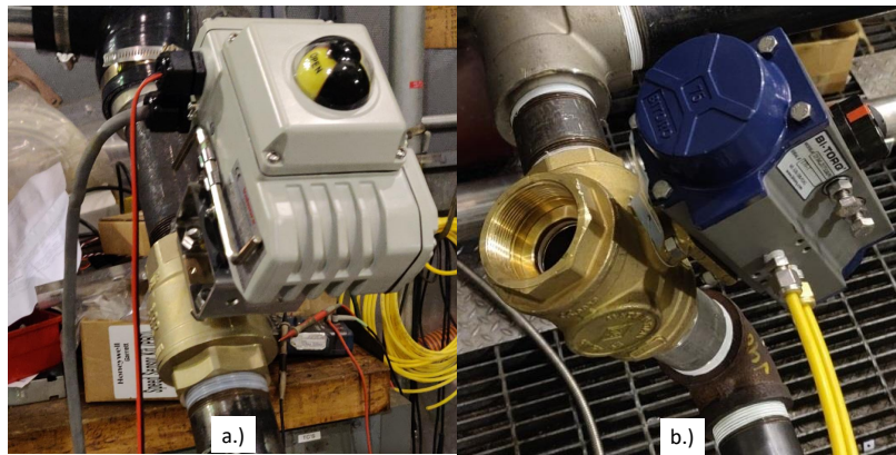
Figure 59. Modifications to Test Stand. a.) Electronic Variable Opening Globe Valve. b.) Pneumatic Three-Way Globe Valve.
