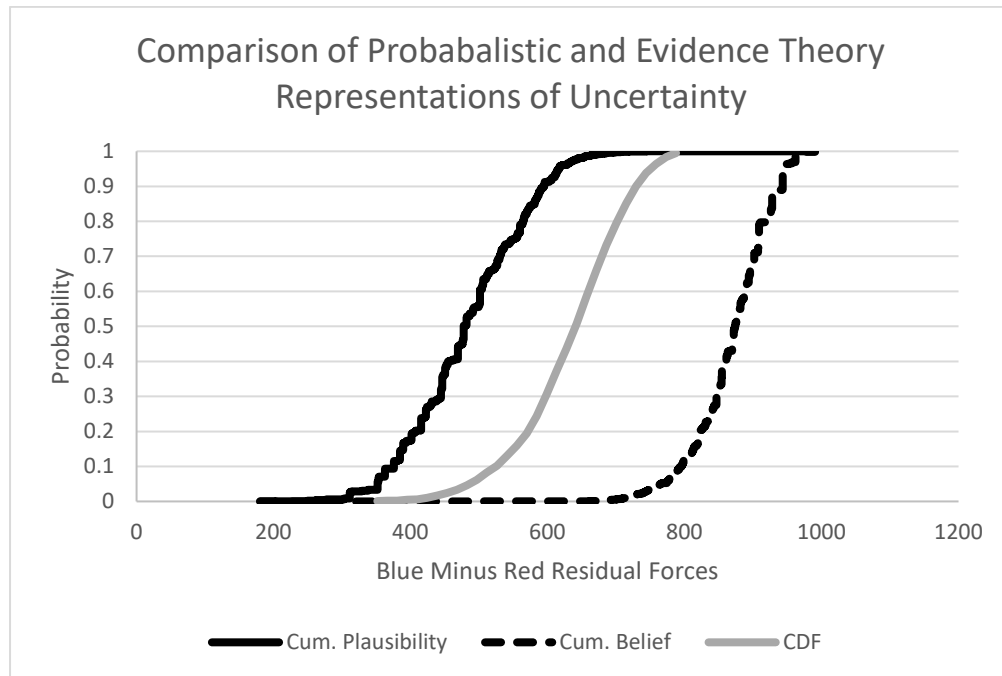
Figure 19: Comparison of Probabilistic and Evidence Theory Representations of Uncertainty
