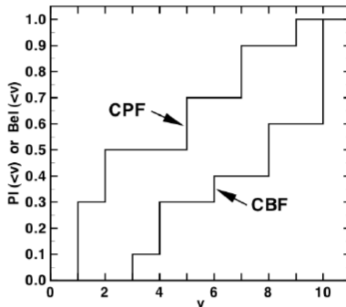
Figure 2: Depiction of Evidence Theory Bounds on CDF (Oberkampff, 2002)
