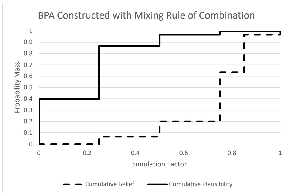
Figure 22: Notional BPA for Representing Uncertain Factors
