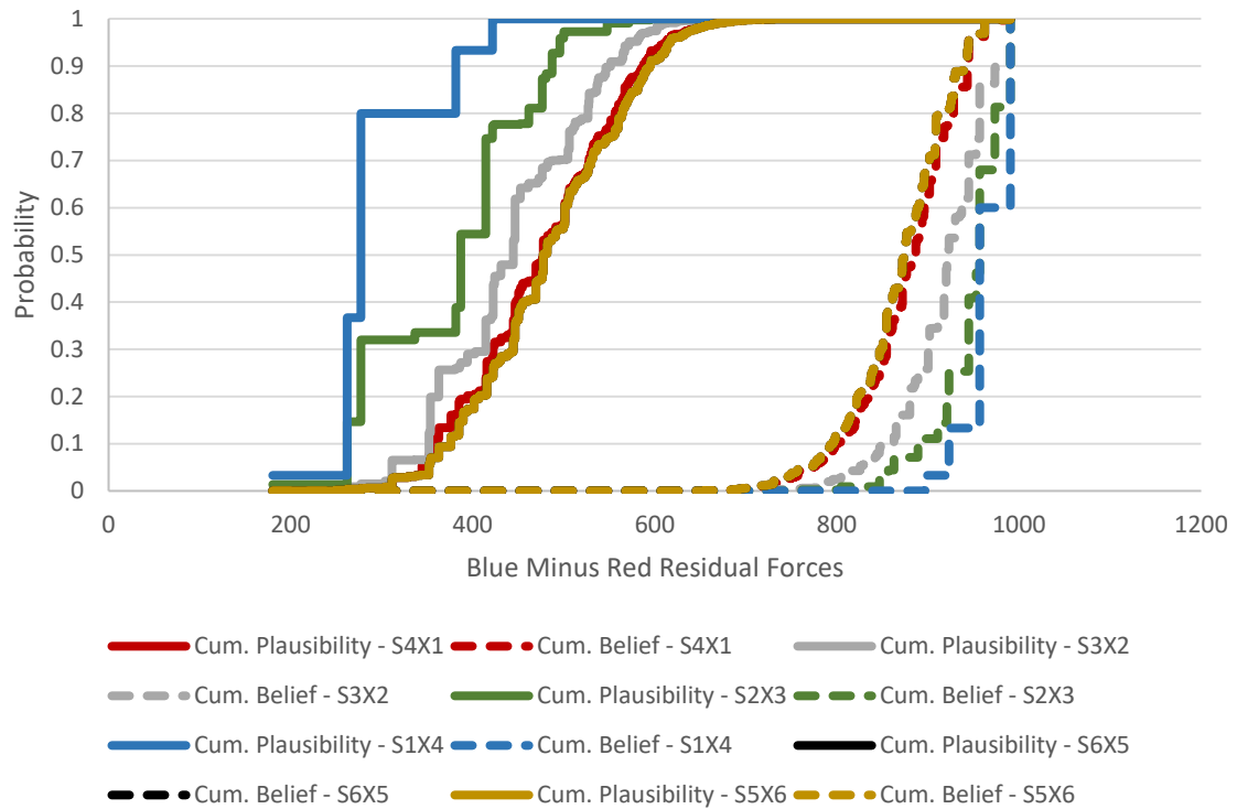
Figure 34: Sensitivity Analysis Summary of Blue minus Red Residual Forces
