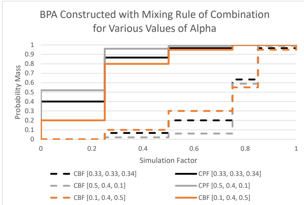
Figure 18: BPAs for Various Relative Weights across Expert Inputs
