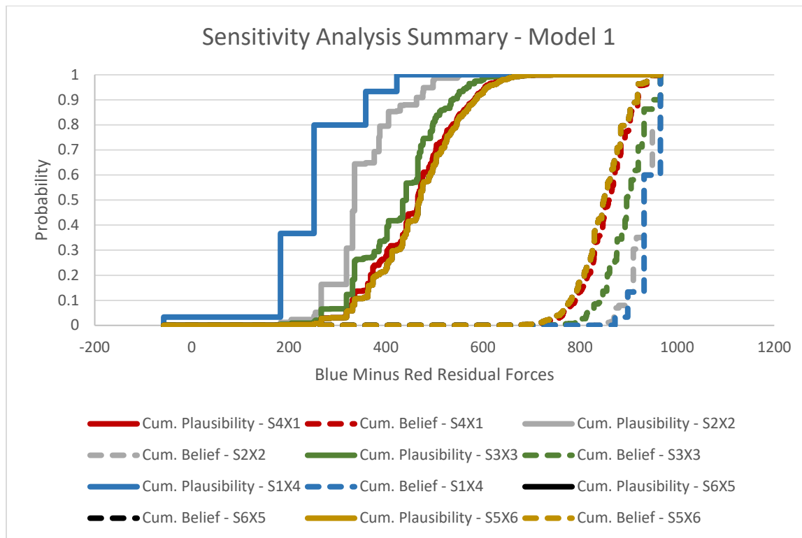
Figure 35: Summary of Uncertain Factor Prioritization for Model 1
