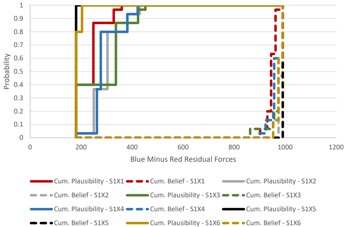
Figure 23: Sensitivity Analysis of Blue minus Red Residual Forces – Step 1
