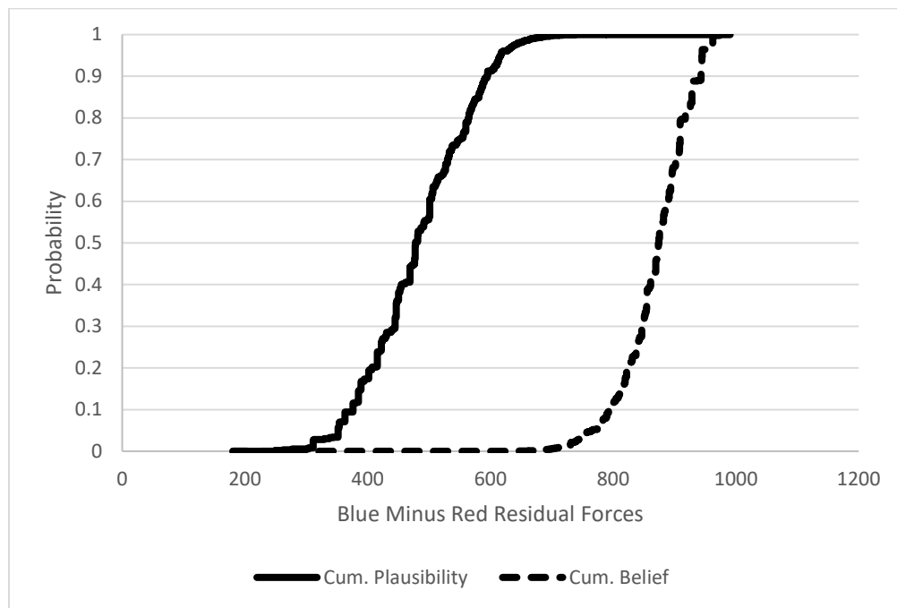
Figure 33: Evidence Theory Representation of Uncertainty
