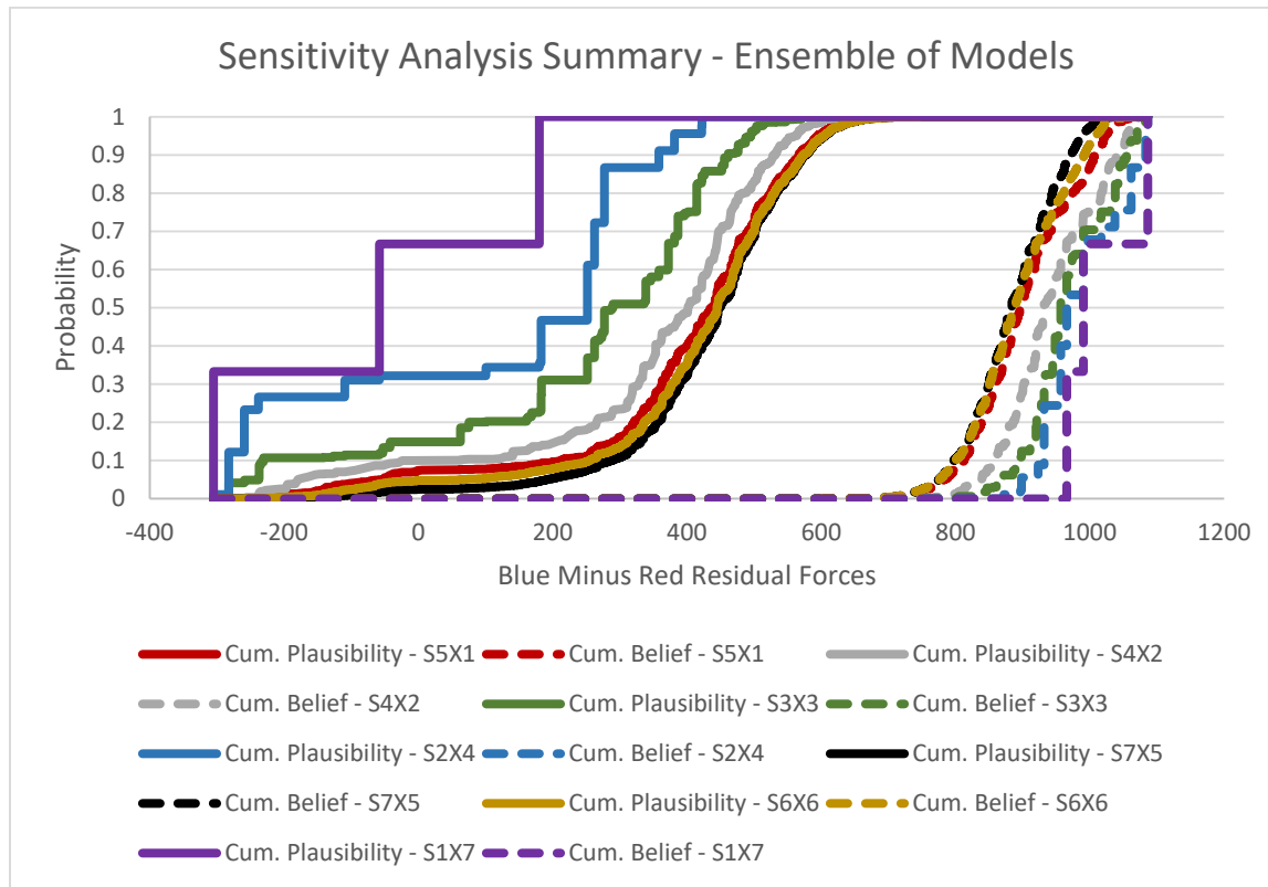
Figure 38: Summary of Uncertain Factor Prioritization for the Ensemble of Models
