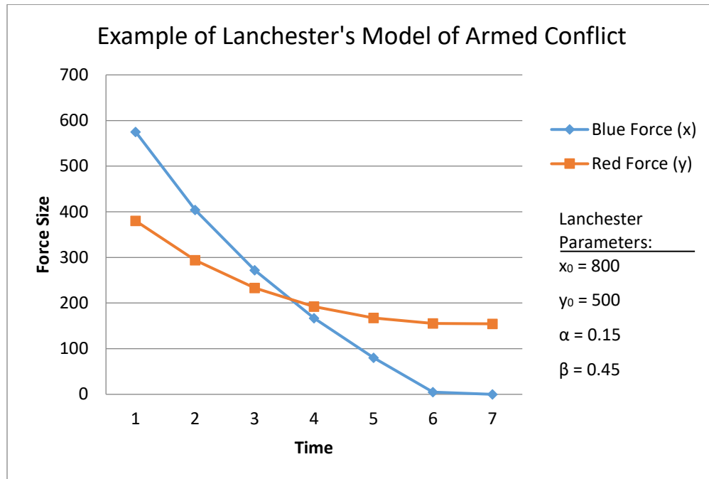
Figure 32: Example of Lanchester's Model of Armed Conflict
