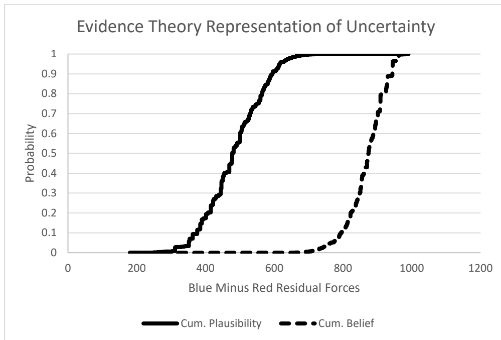
Figure 16: Evidence Theory Representation of Combat Model Uncertainty
