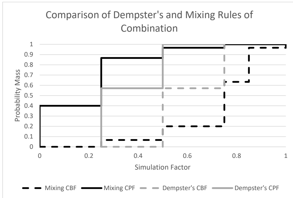
Figure 17: Comparison of Dempster's and the Mixing Rules of Combination
