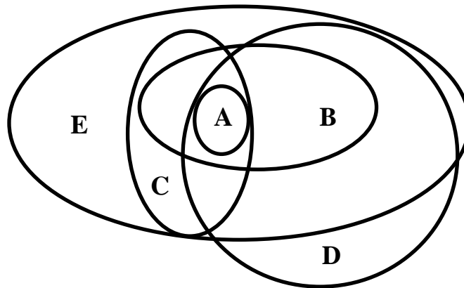
Figure 7: Consistent Evidence
