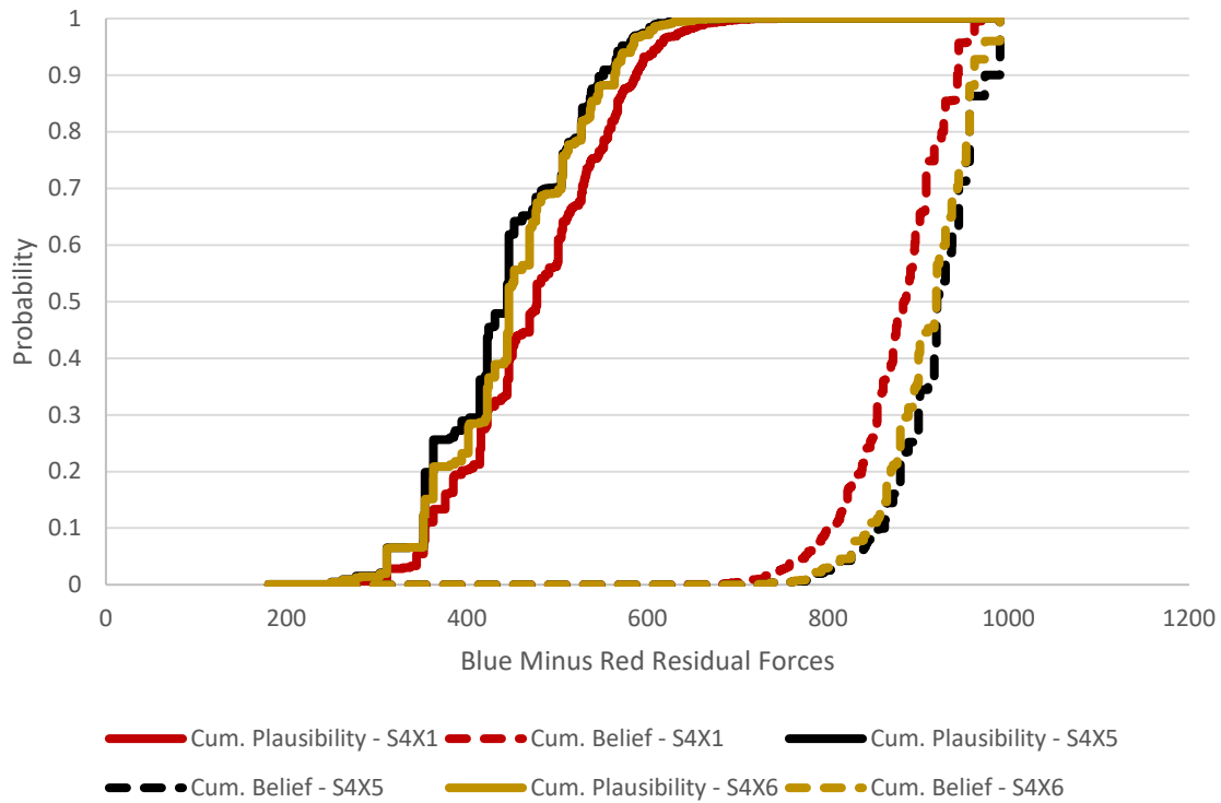
Figure 26: Sensitivity Analysis of Blue minus Red Residual Forces – Step 4
