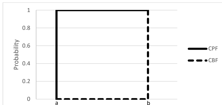
Figure 21: Concept of “Maximum Uncertainty”
