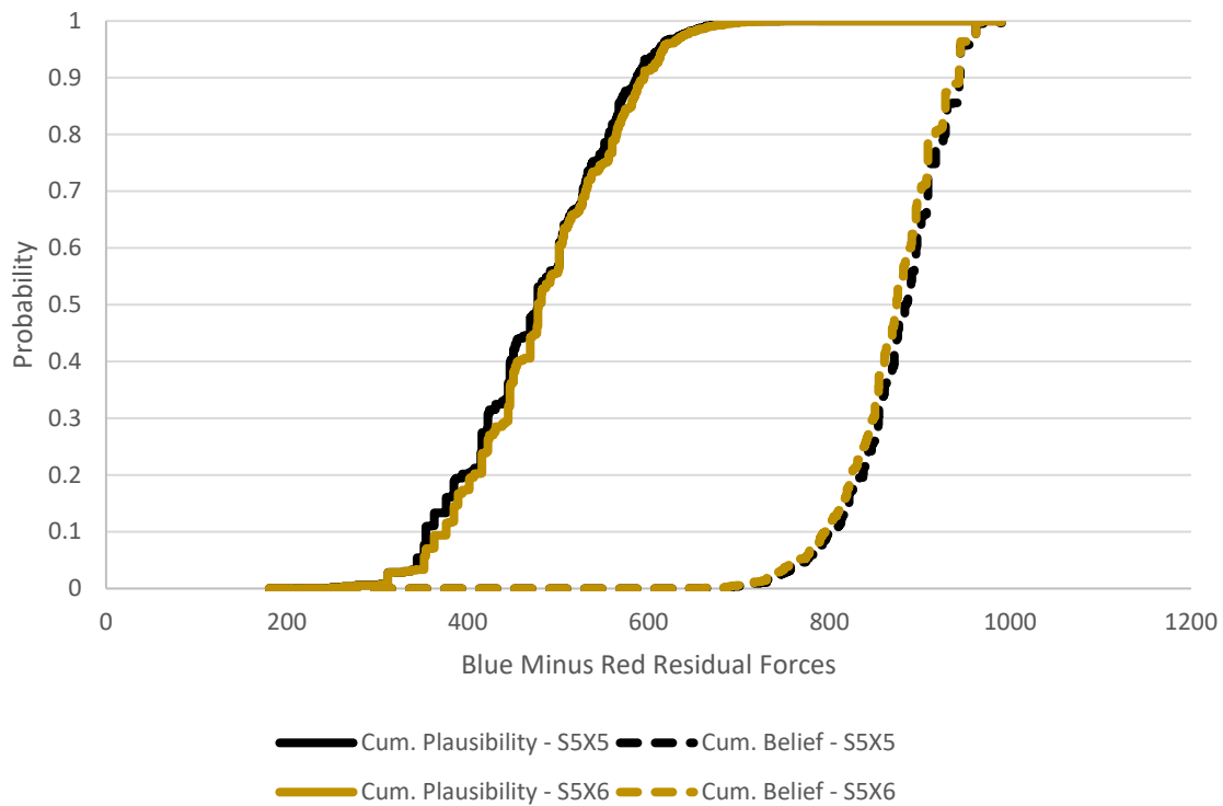
Figure 27: Sensitivity Analysis of Blue minus Red Residual Forces – Step 5
