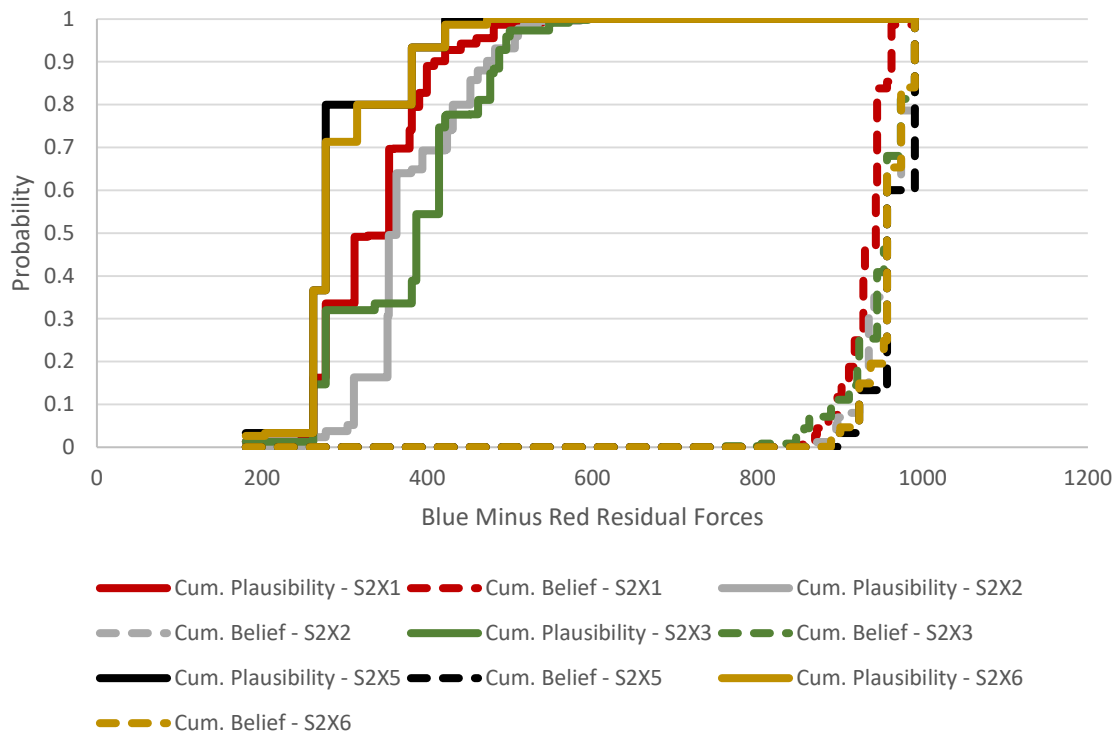
Figure 24: Sensitivity Analysis of Blue minus Red Residual Forces – Step 2
