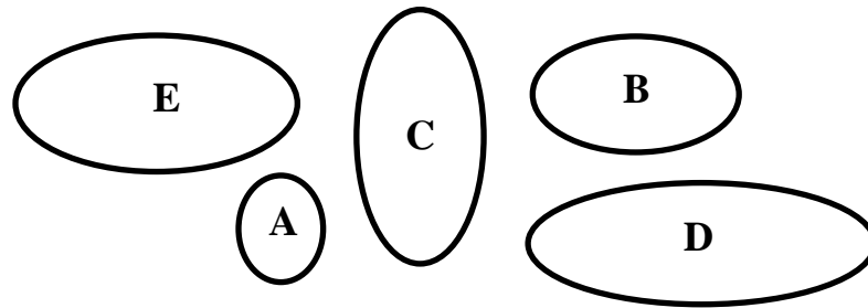
Figure 9: Disjoint Evidence
