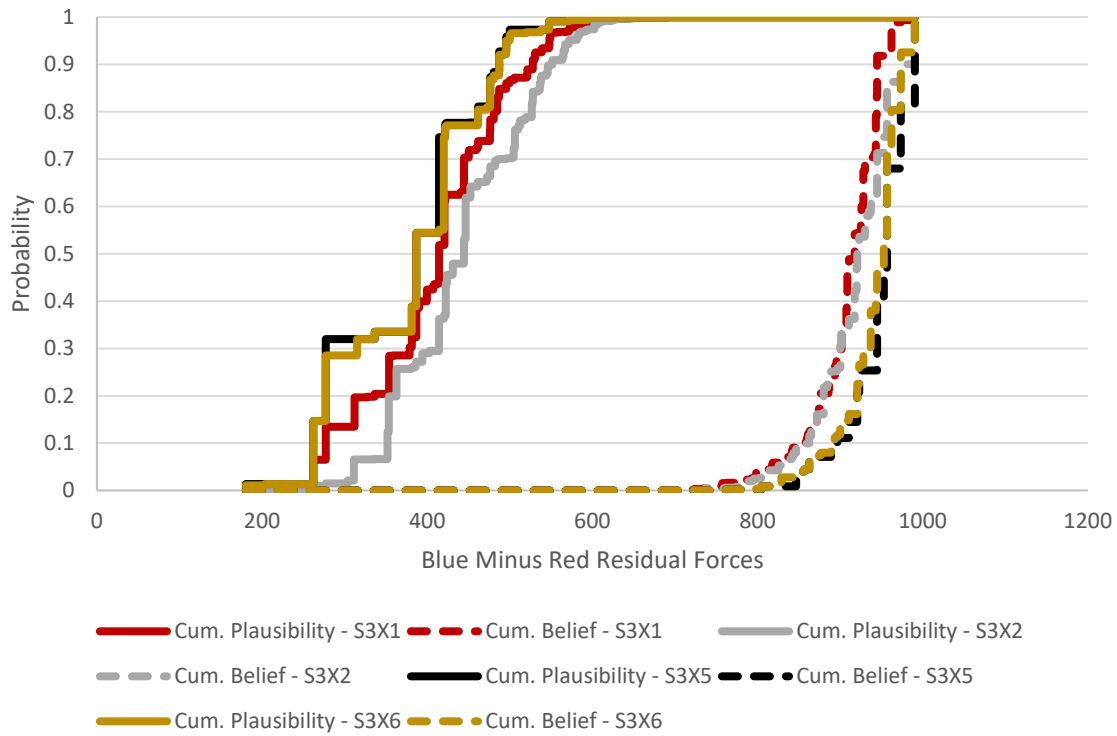
Figure 25: Sensitivity Analysis of Blue minus Red Residual Forces – Step 3
