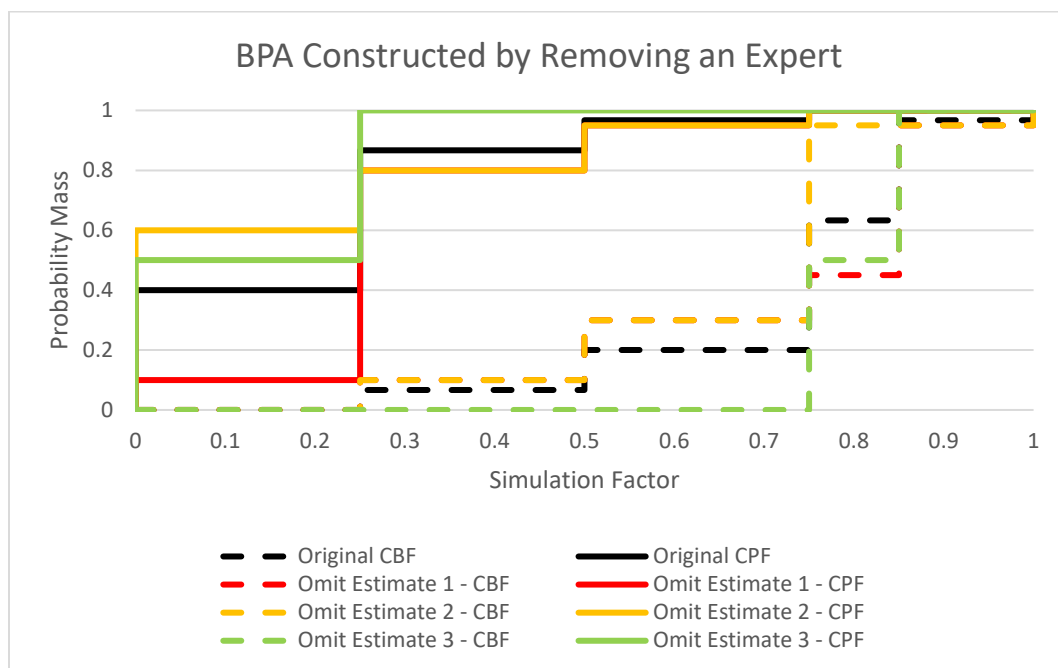
Figure 39: Sensitivity of Factor BPA to Removing an Expert Estimate
