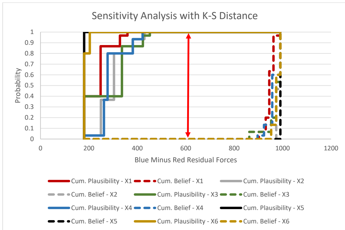
Figure 20: Ties using K-S Distance when Large Uncertainties Exist
