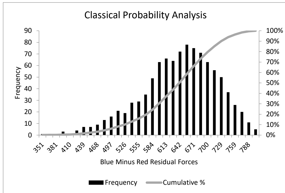
Figure 11: Propagation of Uncertainty via Classical Probability Theory
