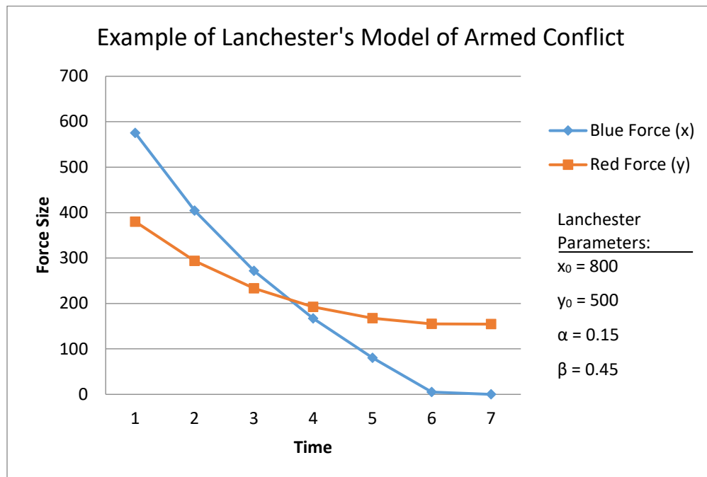
Figure 10: Example of Lanchester's Model of Armed Conflict
