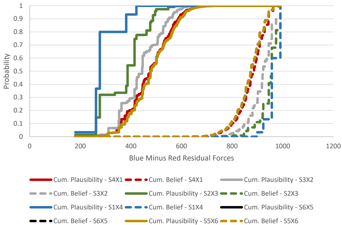
Figure 29: Sensitivity Analysis of Blue minus Red Residual Forces – Summary
