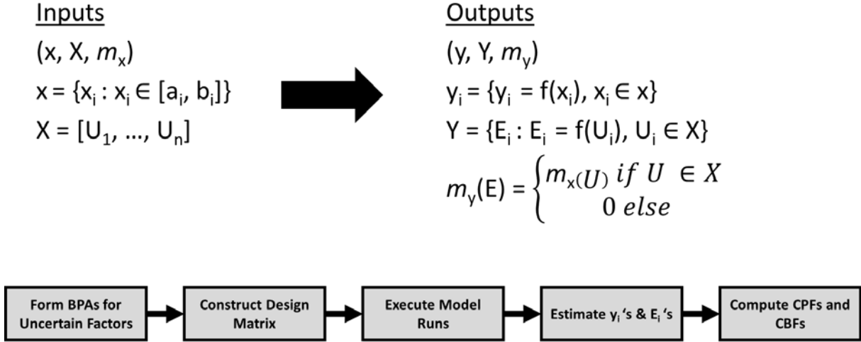
Figure 12: Method for Propagating Uncertain Inputs through Simulation
