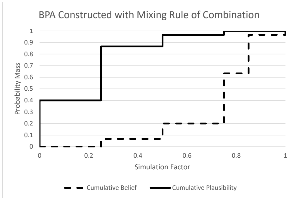
Figure 15: BPA Constructed with Mixing Rule of Combination
