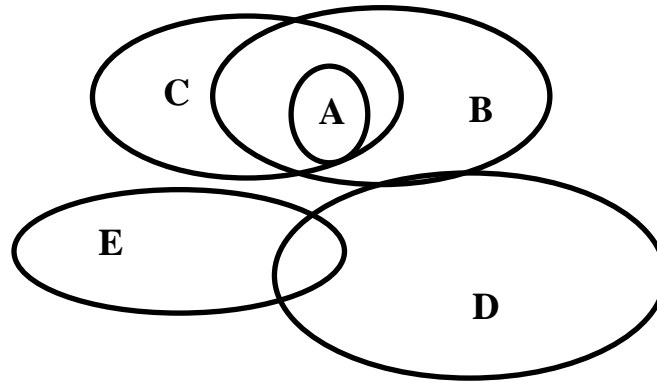
Figure 8: Arbitrary Evidence
