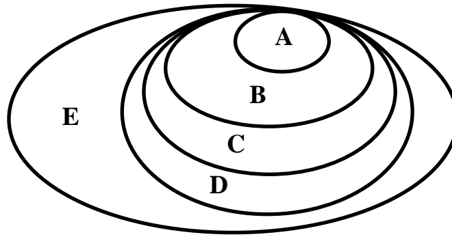
Figure 6: Consonant Evidence
