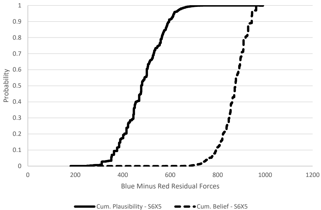
Figure 28: Sensitivity Analysis of Blue minus Red Residual Forces – Step 6
