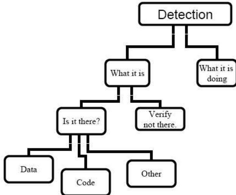
Figure 3.10: Detection Classification 1
