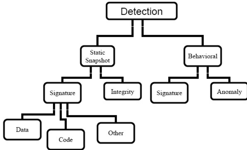
Figure 3.11: Detection Classification 2
